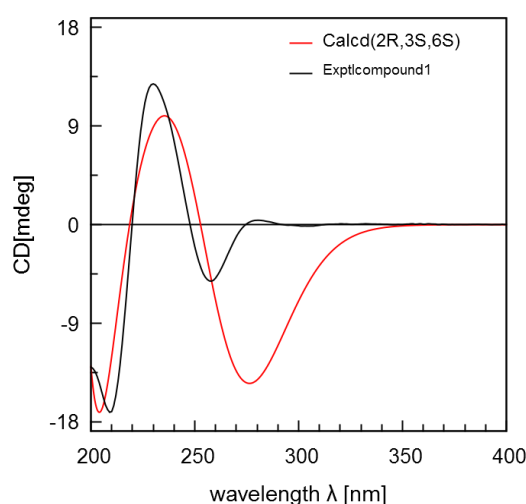
Figure 3. Experimental and calculated ECD spectra of 1 (black line, experimentally recorded in methanol; red line, calculated for 2 R , 3 S , 6 S configuration in methanol).
