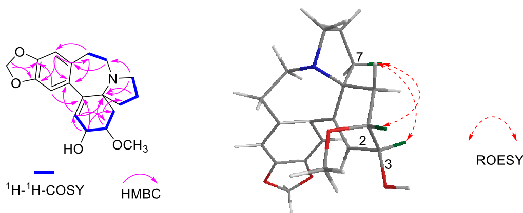
Figure 2. ^1\text{H} – ^1\text{H} COSY correlations and the key HMBC correlations of and the ROESY correlations of compound 1
