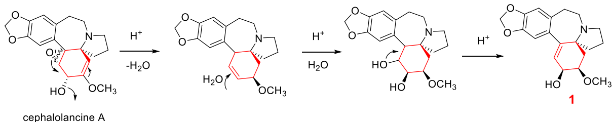
Scheme 1. Proposed biosynthetic pathway of 1 .
