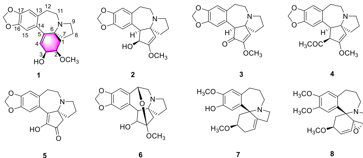
Figure 1. Structures of compounds 1-8
