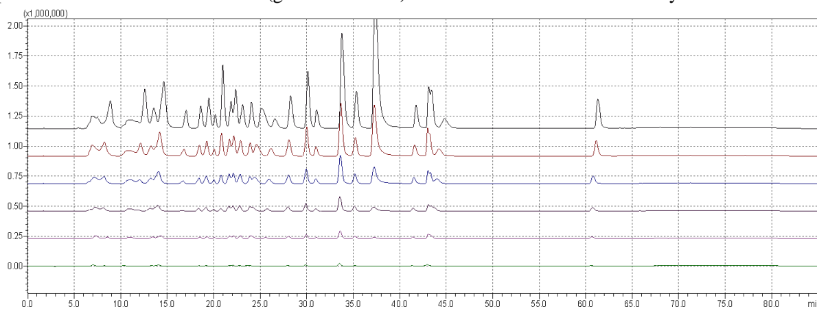
Figure 1. HPLC–DAD chromatograms of 27 phenolic standards at 254 nm: (1) fumaric acid, (2) gallic acid, (3) trans -aconitic acid, (4) p -benzoquinone, (5) pyrocatechol, (6) protocatechuic acid, (7) unknown, (8) 2-(4-hydroxyphenyl) ethanol, (9) 4-hydroxybenzoic acid, (10) (+)-catechin, (11) methyl- p -benzoquinone, (12) 6,7-dihydroxy coumarin, (13) vanillic acid, (14) caffeic acid, (15) vanillin, (16) 2,4-dihydroxybenzoic acid, (17) chlorogenic acid, (18) p -coumaric acid, (19) ferulic acid, (20) coumarin, (21) trans -2-hydroxycinnamic acid, (22) rutin, (23) ellagic acid, (24) trans -cinnamic acid, (25) naringenin, (26) quercetin, (27) rosmarinic acid, (28) chrysin. Inertsil ODS-3 column (4 \mu m, 4 mm x 150 mm). Mobile phase 0.1% acetic acid-methanol (gradient elution). Flow rate 1 mL/min. Diode array detection 254 nm.
