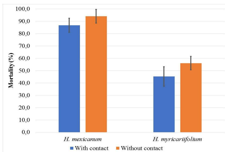
Figure 2. Fumigant activity results of "vial in vial" methods with and without contact
