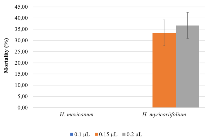
Figure 3. Contact toxicity results against S. zeamais of EO from active species of the Hypericum genus
