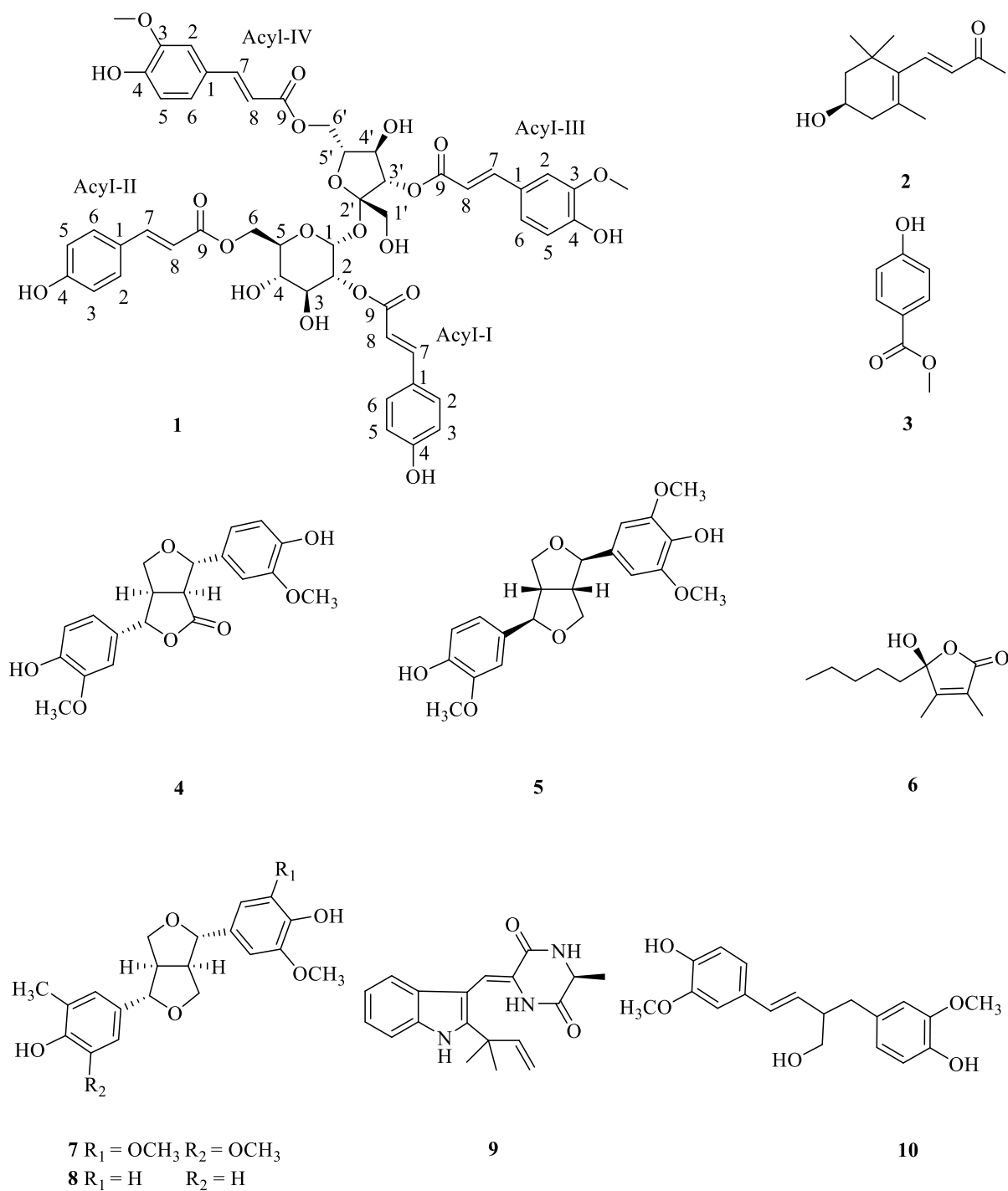
Figure 1. Structures of 1–10
