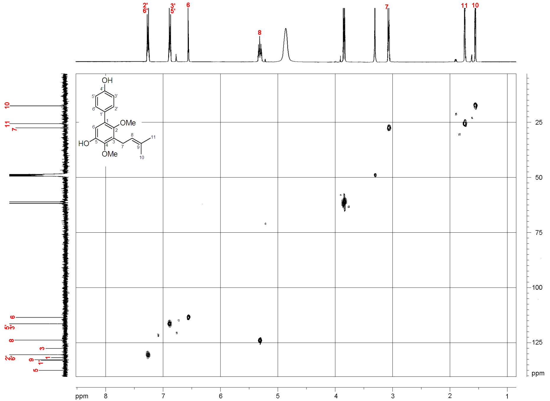
S3: HSQC spectrum of multiflorabiphenyl A (1)
