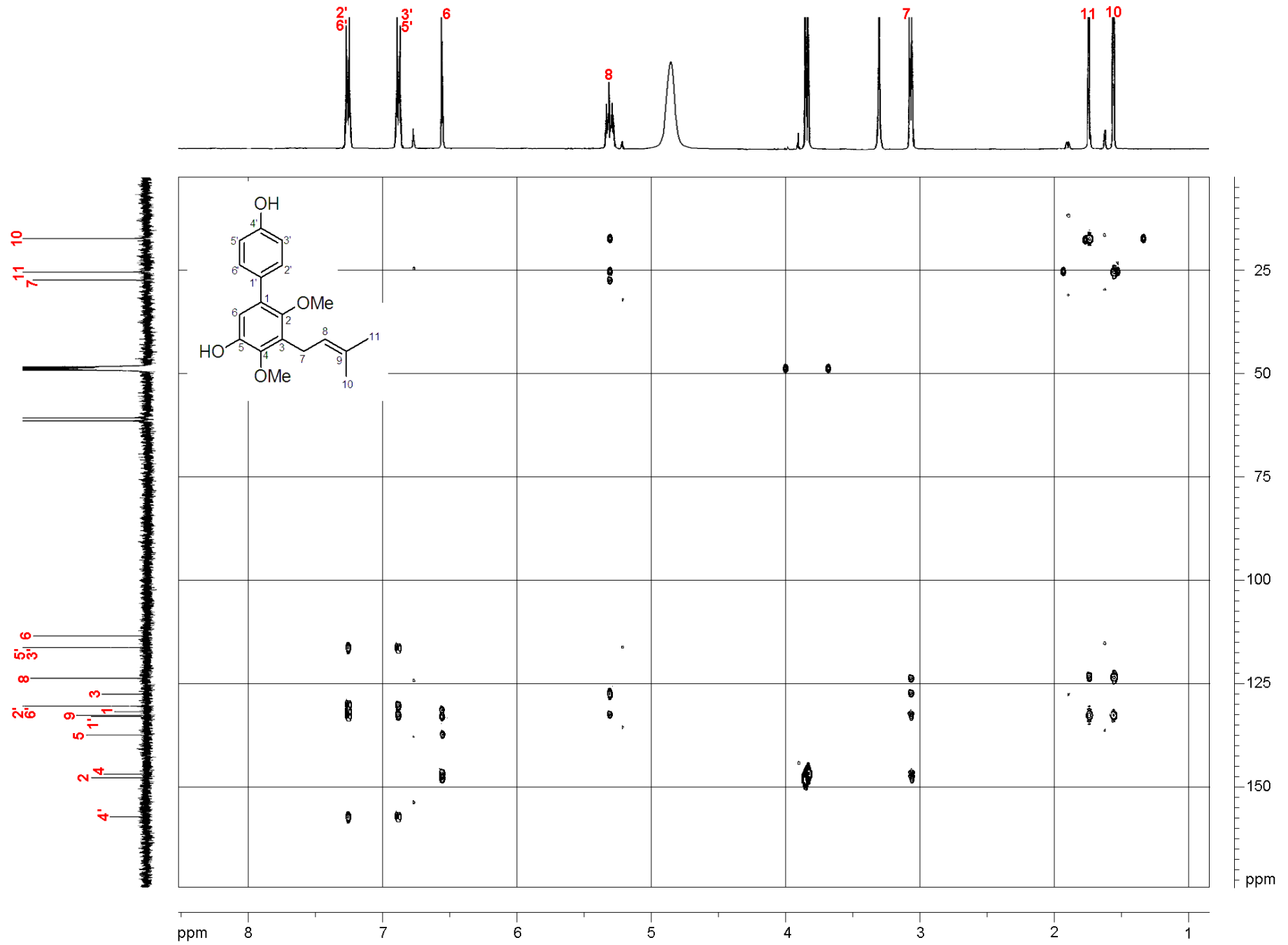
S4: HMBC spectrum of multiflorabiphenyl A (1)
