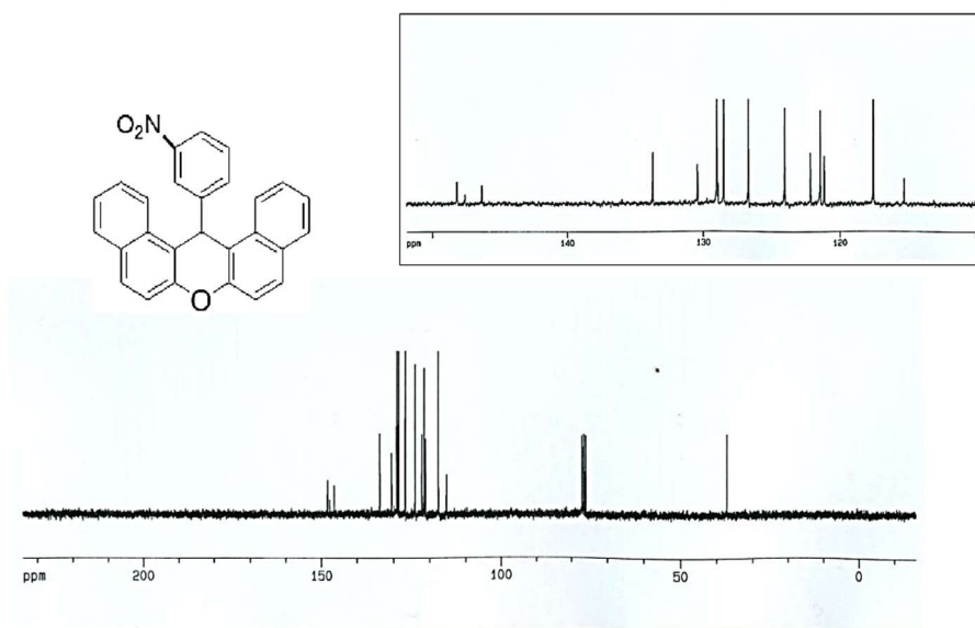
Figure S5. 100 MHz 13 C-NMR spectrum of 2e
