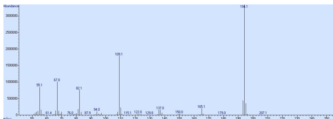
Figure S1. Mass spectrum of caffeine.
