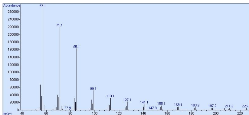
Figure S2. Mass spectrum of n-docosane (IS)
