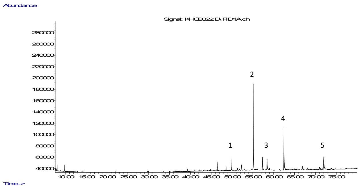
Figure S2 : Chromatogram of main compounds of Crataegus azaroulus dry inflorescences and immature fruits- Cengizköy-Lefke / Sample B (1: Eicosane, 2: Tricosane, 3: Tetracosane, 4: Pentacosane, 5: Heptacosane)
