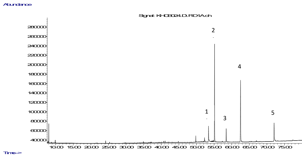
Figure S3 : Chromatogram of main compounds of Crataegus pallasii dry inflorescences and immature fruits- Bata Region-Libya / Sample C (1: Carvacrol, 2: Tricosane, 3: Tetracosane, 4: Pentacosane, 5: Heptacosane)
