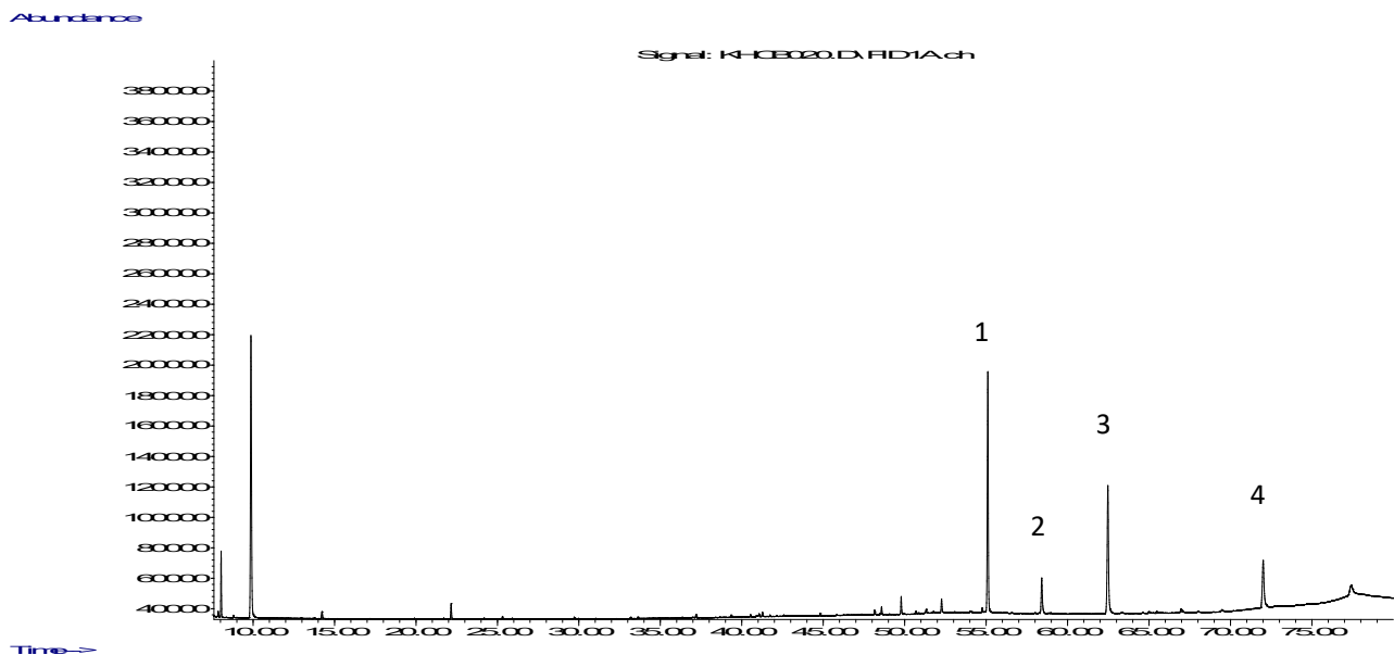
Figure S1 : Chromatogram of main compounds of Crataegus azaroulus fresh inflorescences and immature fruits- NEU Campus / Sample A (1: Tricosane, 2: Tetracosane, 3: Pentacosane, 4: Heptacosane)
