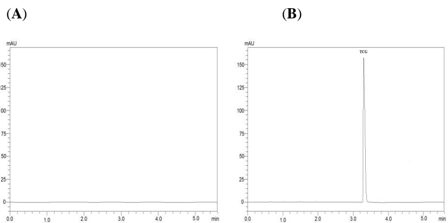
Figure S1: Representative chromatograms of (A) blank , (B) TCG spiked with 50 \mu\text{g/mL}
