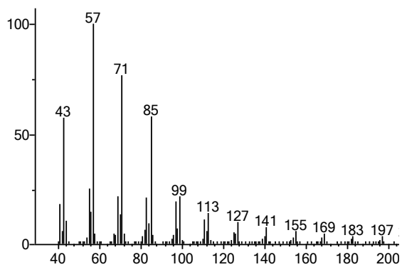
Figure S2: MS spectrum of unidentified compound 2
