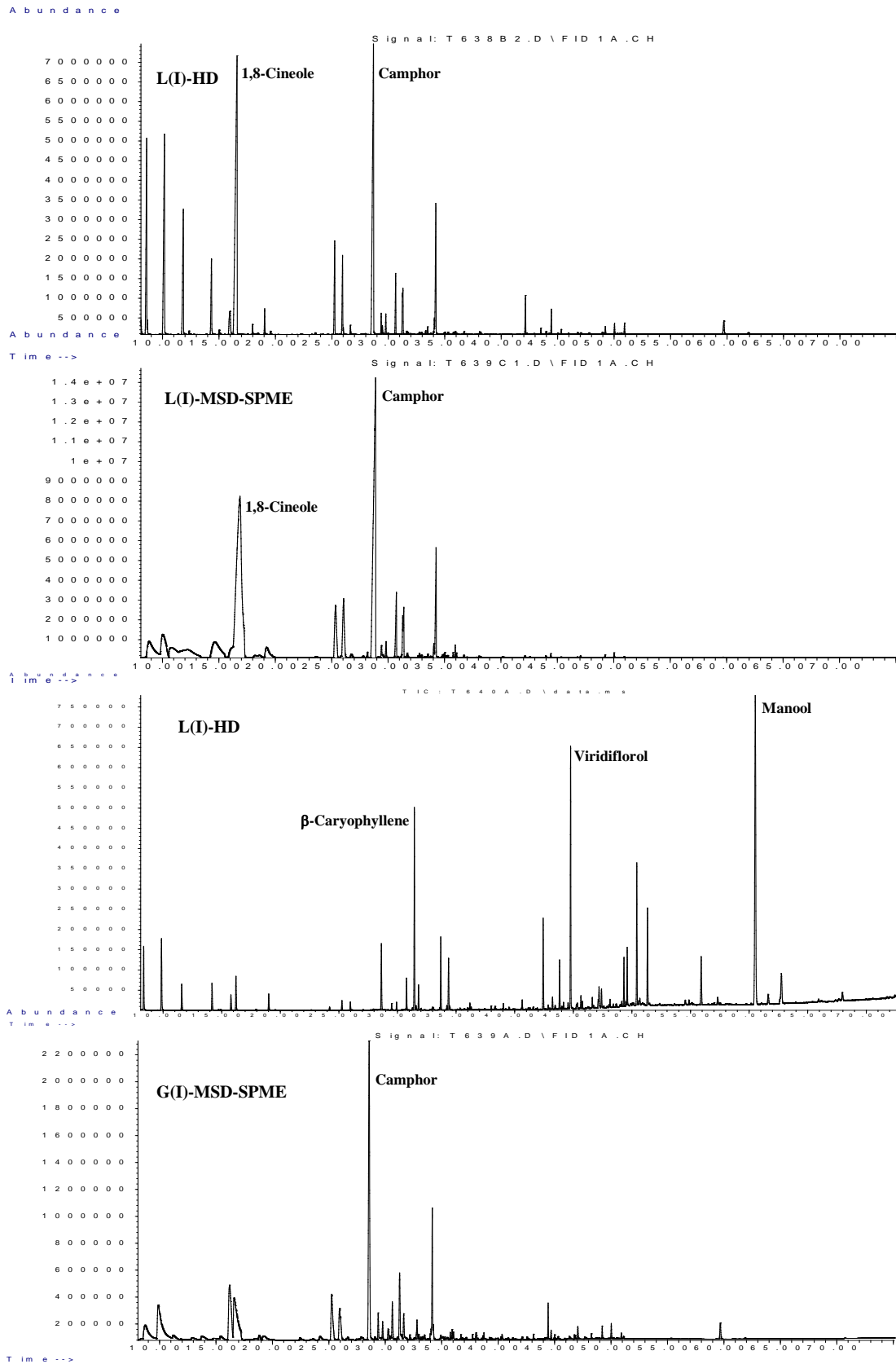
Figure S2 : Chromatographic profile of the volatiles obtained with hydrodistillation (HD) and MSD-SPME techniques from the leaves (L) and the galls (G) of S. fruticosa
