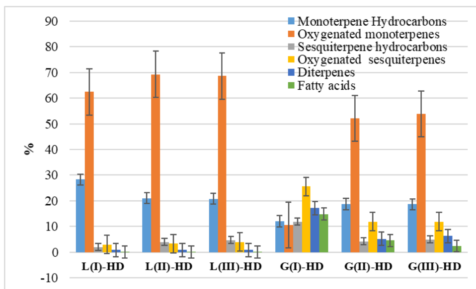
Figure S1. Distribution of the major compound groups in the leaf (L) and gall (G) oils of S. fruticosa obtained with hydrodistillation (HD).
