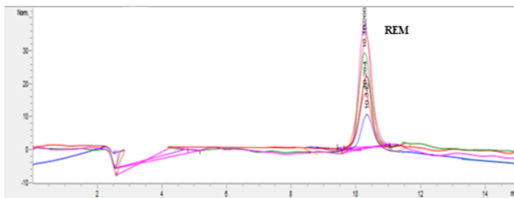
Figure S5: Overlay Chromatogram of Remogliflozin etabonate (Methanol :Water, 70:30% v/v)
