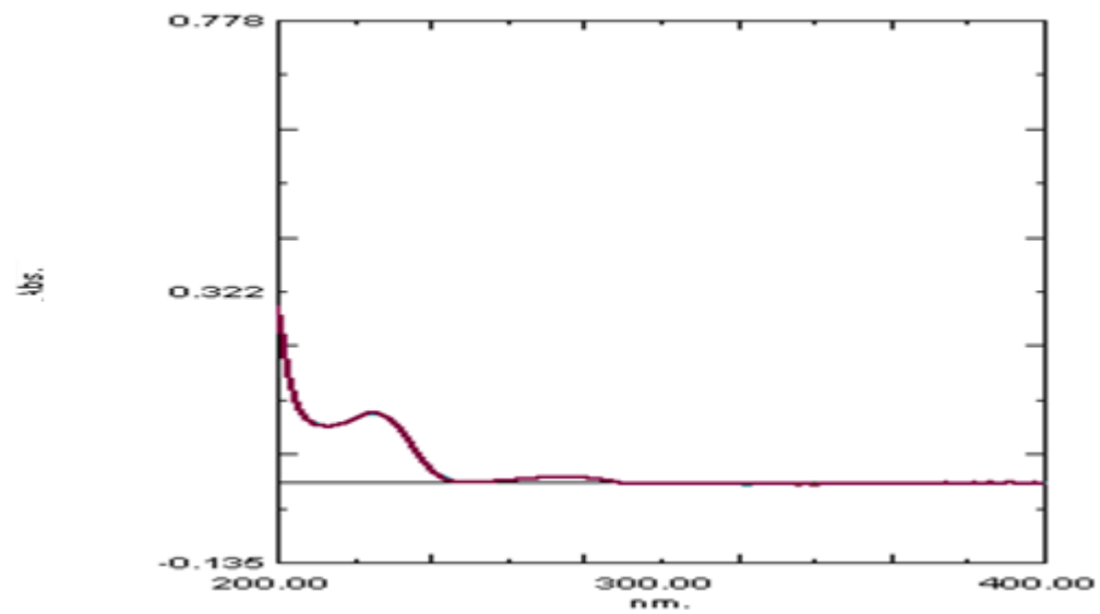
Figure S2: UV Spectra of Remogliflozin etabonate 10µg/mL in methanol.
