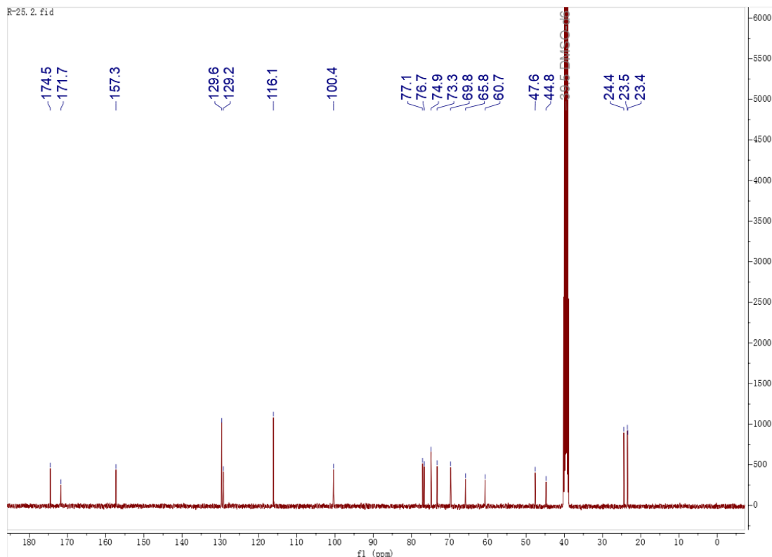
Figure S14: ^{13}\text{C} -NMR (100 MHz, \text{DMSO-}d_6 ) spectrum of 7 (gymnoside II) ^{13}\text{C} -NMR (100 MHz, \text{DMSO-}d_6 ) \delta : 171.7 (C-1), 74.9 (C-2), 44.8 (C-3), 174.5 (C-4), 47.6 (C-5), 24.4 (C-6), 23.5 (C-7), 23.4 (C-8), 129.2 (C-1'), 129.6 (C-2', 6'), 116.1 (C-3', 5'), 157.3 (C-4'), 65.8 (C-7'), 100.4 (C-1''), 73.3 (C-2''), 76.7 (C-3''), 69.8 (C-4''), 77.1 (C-5''), 60.7 (C-6'').
