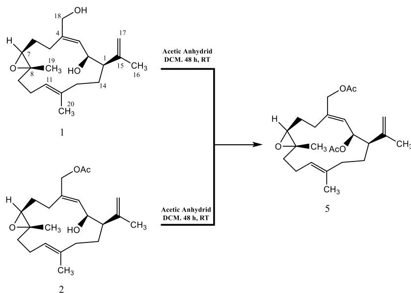
Figure 4. Acetylation of 1 and 2 with acetic anhydride
