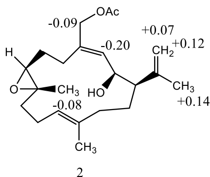
Figure 2. Chemical shifts differences between R and S -MPA esters of compound 2
