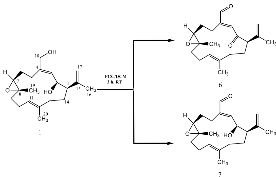
Figure 5. Oxidation of 1 with PCC
