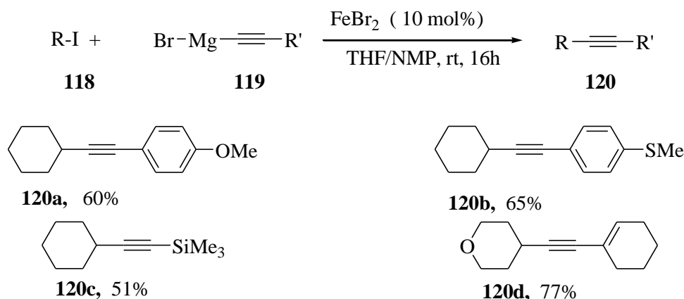
Scheme 14. Coupling reaction of secondary alkyl halides with alkynyl Grignard reagent using \text{FeBr}_2
