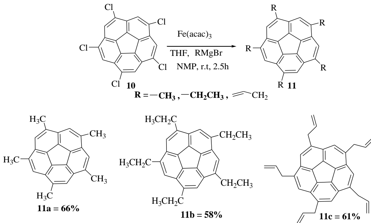
Scheme 3. Fe(acac) 3 catalyzed cross-coupling of 10 with various alkylmagnesium bromides
