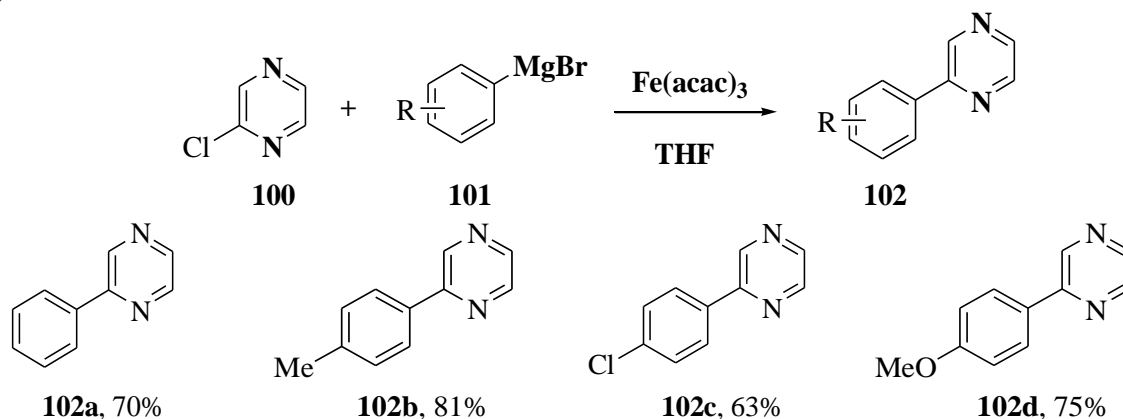
Scheme 9. Coupling of 2-chloropyrazine with aryl Grignard reagents catalyzed by \text{Fe}(\text{acac})_3 (0.5 mol%)
