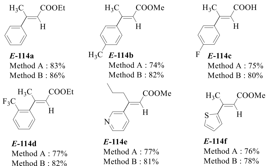
Scheme 13. E -trisubstituted acrylates using method A and B
