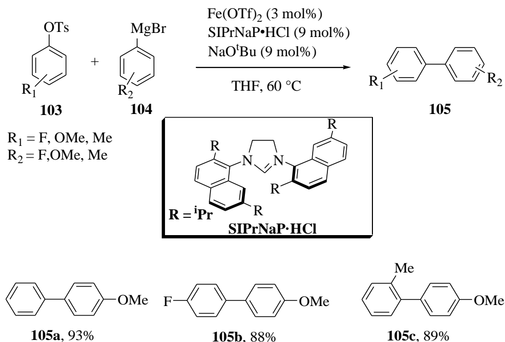
Scheme 10. Cross-coupling of aryl tosylates and arylmagnesium reagents using Fe(OTf) 2 /SIPrNaP·HCl/NaOtBu
