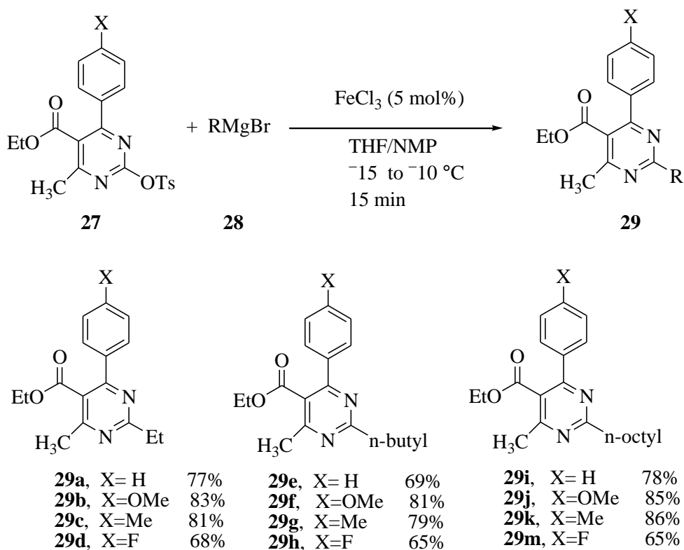
Scheme 4. Iron-catalyzed cross-couplings of pyrimidin-2-yl tosylates with alkylmagnesium reagents
