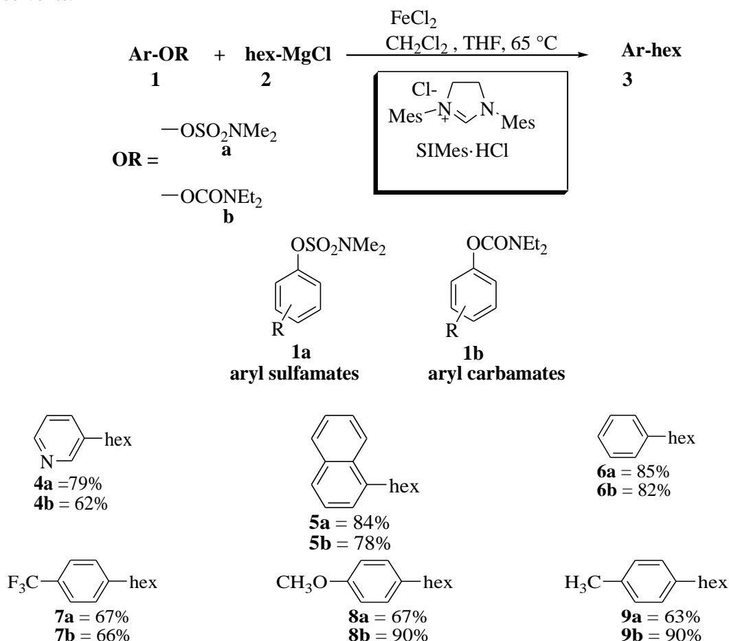
Scheme 2. Coupling reaction of aryl carbamates and sulfamates with n-hexylmagnesium chloride using iron catalyst
