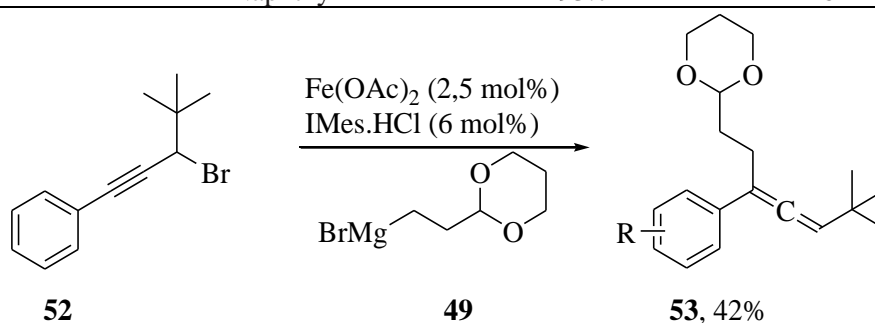
Scheme 5. Reaction of tert -butyl-substituted propargyl bromide is regioselective
