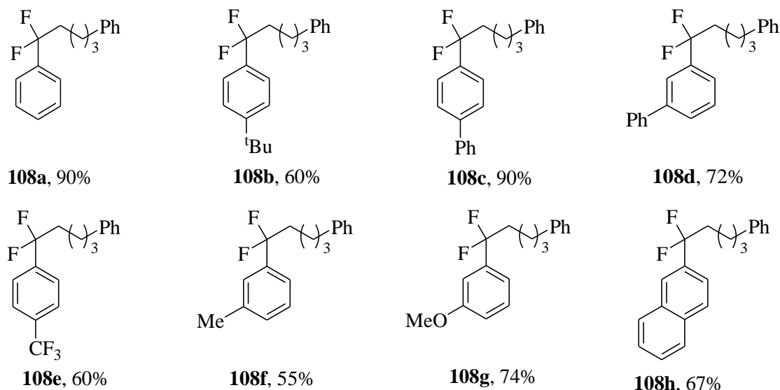
Scheme 11. Fe-catalyzed difluoroalkylations of arylmagnesium bromides with difluoroalkyl bromides
