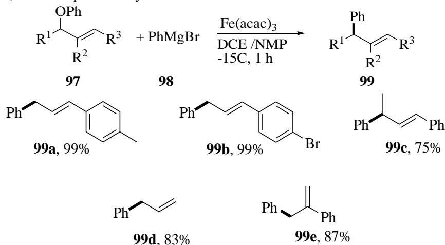
Scheme 8. \text{Fe}(\text{acac})_3 catalyzed coupling of various allylic ethers with phenylmagnesium bromide
