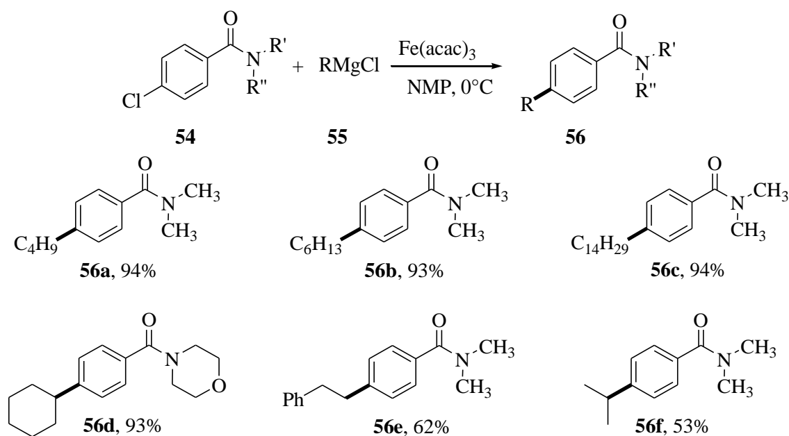
Scheme 6. Iron-catalyzed cross-coupling of amides with alkylmagnesium reagents
