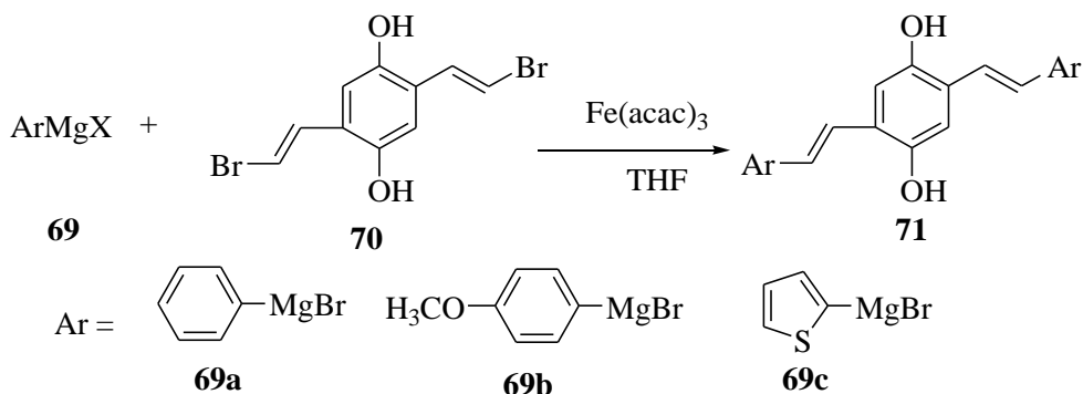
Scheme 7. Iron catalyzed cross-coupling reaction leading to bis(2-arylvinyl)benzenes
