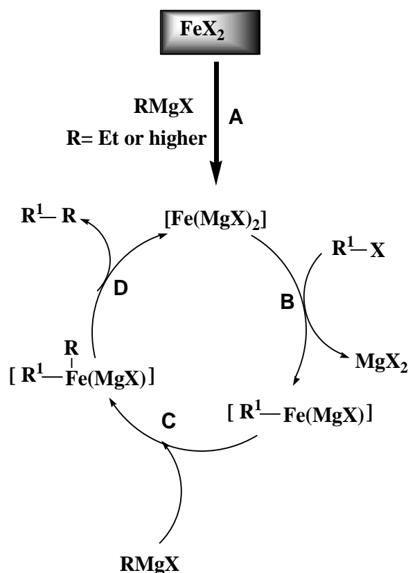
Scheme 1. The general mechanism of iron catalyzed cross-coupling organomagnesium with substrates
