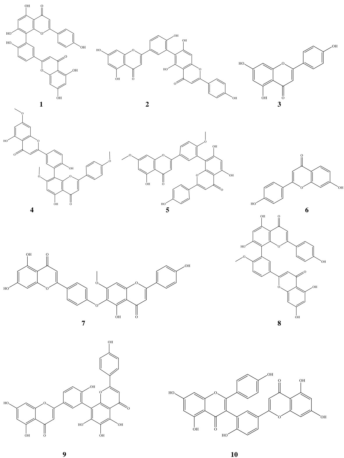
Figure 1. Major flavonoids identified from Selaginella . (1) Amentoflavone, (2) Robustaflavone, (3) Apigenin, (4) Heveaflavone, (5) Ginkgetin, (6) 4',7 – Dihydroxyflavone, (7) Isocryptomerin (8) Bilobetin (9) Sumaflavone, (10) Taiwaniaflavone
