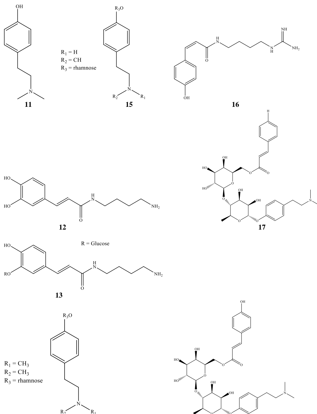
Figure 2. Major alkaloids identified from Selaginella . (11) Hordenine, (12) Paucine, (13) Paucine-3-β-D-glucopyranoside, (14) Hordenine-O-α-rhamnopyranoside, (15) N-methyltyramine-O-α-rhamnopyranoside, (16) N¹-cis-p-coumaroylagmatine, (17) Hordenine-O-[(6-O-cinnamoyl)-O-β-glucopyranosyl]-α-rhamnopyranoside, (18) Hordenine-O-[(6-O-p-coumaroyl)-O-β-glucopyranosyl]-α-rhamnopyranoside
