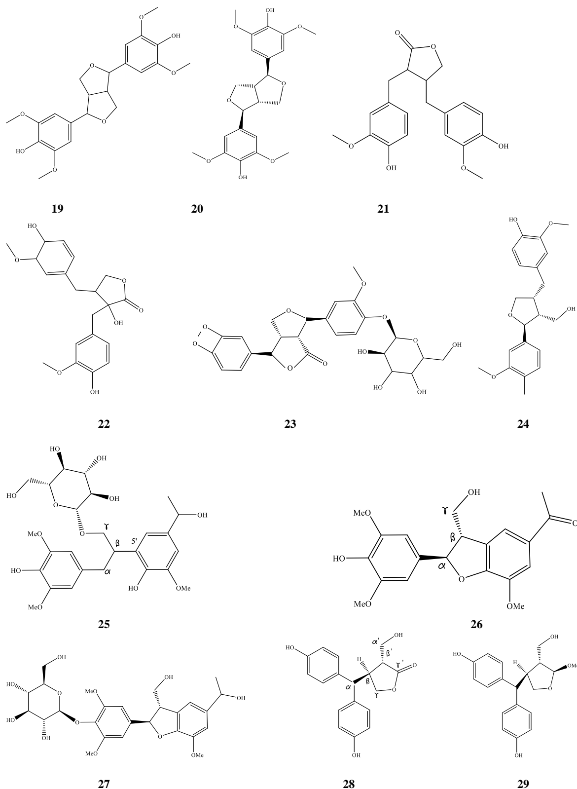
Figure 3. Major lignans identified from Selaginella . (19) (–)-Lirioresinol A, (20) (+)-Syringaresinol, (21) (+)-Matairesinol, (22) Wikstromol, (23) Styralignolide B, (24) (+)-Lariciresinol, (25) Tamariscinoside B (26) (2 R ,3 S )- Dihydro-2-(3,5-dimethoxy-4-hydroxyphenyl)-7-methoxy-5-acetyl-benzofuran (27) Tamariscinoside C (28) 3,4- trans -3-hydroxymethyl-4-[bis(4-hydroxyphenyl)methyl]butyrolactone, (29) 2,3- trans -3,4- trans -2-methoxy-3-hydroxymethyl-4-[bis(4-hydroxyphenyl)methyl]tetrahydrofuran.
