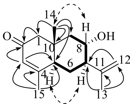
Figure 2. ^1\text{H} - ^1\text{H} COSY (—), HMBC (→), and NOE (↔) correlations of 1 .
