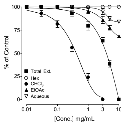
Figure 2. Concentration-dependent inhibitory effects of the total extract of P. mahaleb Total Ext., Hex, \text{CHCl}_3 , EtOAc and Aqueous fractions against carbachol (CCh; 1 \mu\text{M} )-induced contractions in isolated guinea-pig tracheal preparations. Symbols represent mean \pm SEM; n= 4-5.
