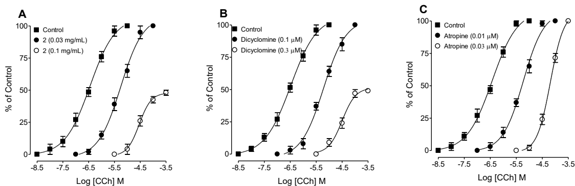
Figure 5: Concentration-response curves of carbachol (CCh) in the absence and presence of the increasing concentrations of the (A) 2 , (B) dicyclomine and (C) atropine in isolated guinea-pig tracheal preparations. Symbols represent mean ± SEM; n= 4-5.
