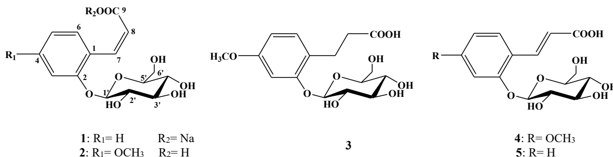
Figure 1. Structure of compounds 1- 5
