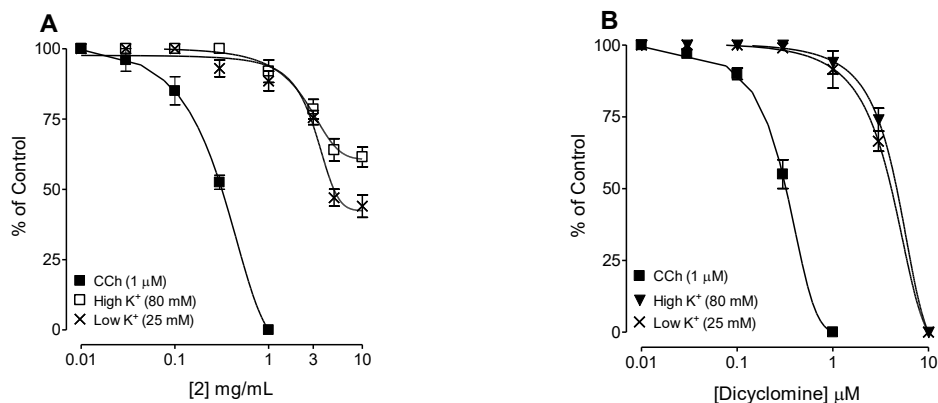
Figure 4: Concentration-dependent inhibitory effects of the (A) 2 and (B) dicyclomine against carbachol (CCh; 1 μM), low K + (25 mM) and high K + (80 mM)-induced contraction in isolated guinea-pig tracheal preparations. Symbols represent mean ± SEM; n= 4-5.
