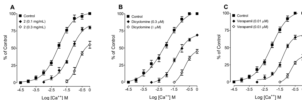
Figure 6. Concentration-response curves of Ca^{2+} in the absence and presence of the increasing concentrations of the (A) 2 , (B) dicyclomine and (C) verapamil in isolated guinea-pig tracheal preparations. Symbols represent mean \pm SEM; n = 4-5 .
