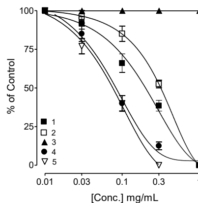
Figure 3. Concentration-dependent inhibitory effects of 1-5 . isolated from chloroform fraction of the P. mahaleb against carbachol (CCh; 1 \mu\text{M} )-induced contractions in isolated guinea-pig tracheal preparations. Symbols represent mean \pm SEM; n= 4-5.
