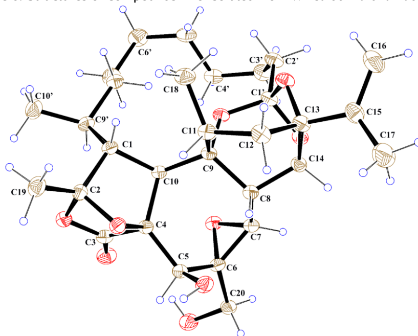
Figure 7. ORTEP diagram of pimelotide A (7)
