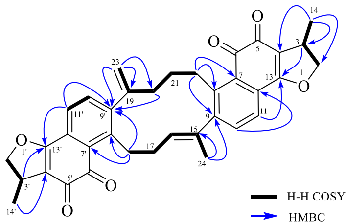
Figure 2. Key HMBC (arrows) and ^1\text{H} - ^1\text{H} COSY (bold) correlations of 1
