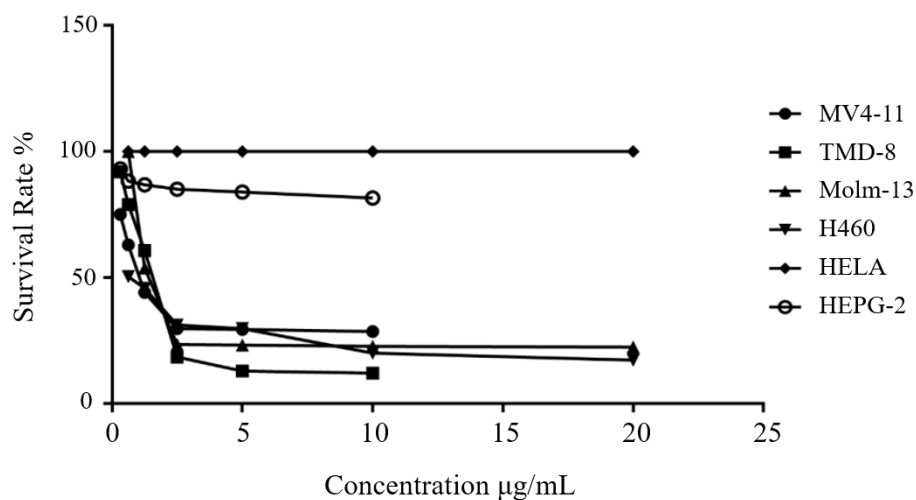
Figure 4. Growth inhibition curves of 1 on MV4-11, TMD-8, MOLM-13, H460, HepG-2, and HeLa cells (72 hours)
