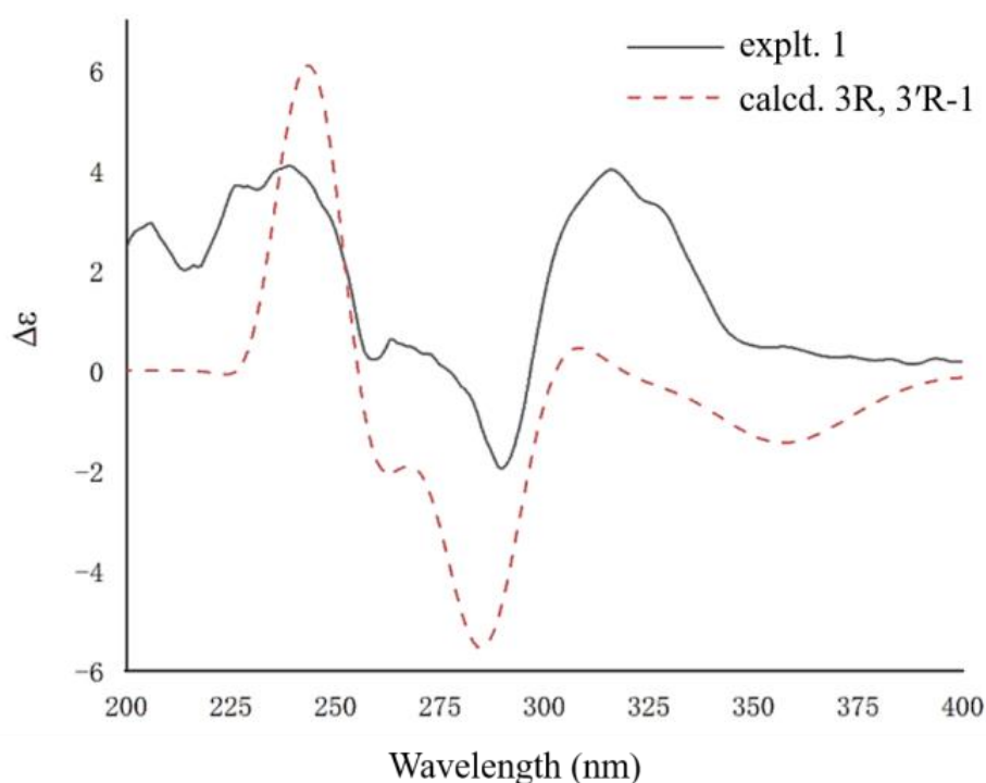
Figure 3. Calculated ECD curve and experimental ECD spectrum of 1
