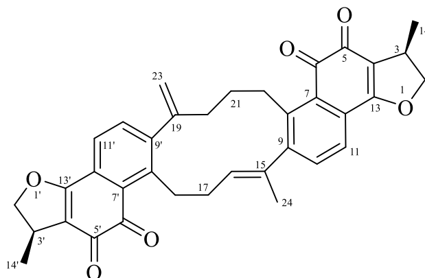
Figure 1. Chemical structure of compound 1
