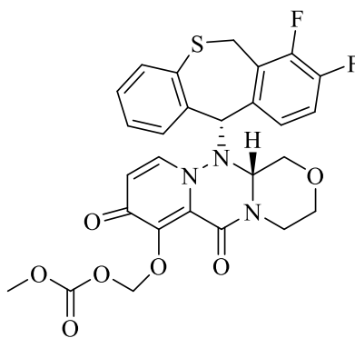
Figure 1. Chemical structure of Baloxavir marboxil
