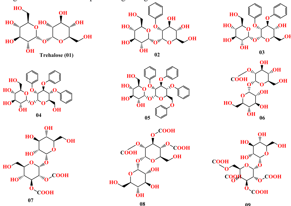
Figure 1. Chemical structure of Trehalose and its derivatives
