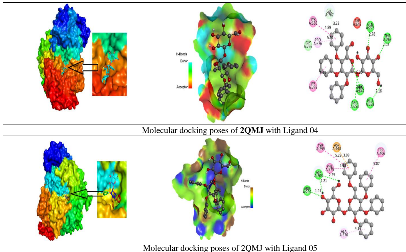
Figure 3. Molecular docking poses and 2d structure of protein of diabetes mellitus
