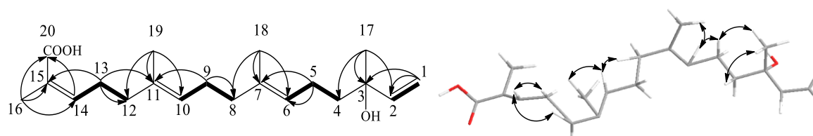
Figure 2. The ^1\text{H} - ^1\text{H} COSY (bold lines), key HMBC (arrows), and NOESY (double head arrows) correlations of compound 1
