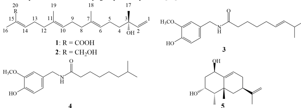
Figure 1. The chemical structures of the compounds 1–5 isolated from C. frutescens L.
