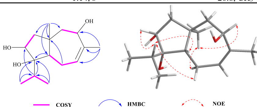
Figure 2. Key 1 H- 1 H-COSY, HMBC, and NOE correlations for 1
