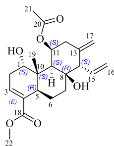
Figure 1. Chemical structure of incarnatin A ( 1 )
