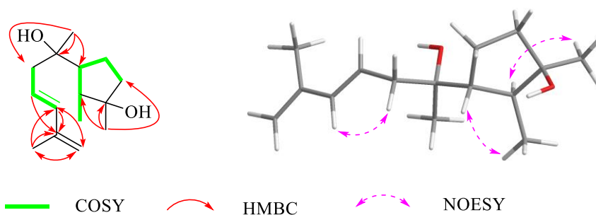
Figure 2. Key ^1\text{H} - ^1\text{H} -COSY, HMBC, and NOE correlations for 1
