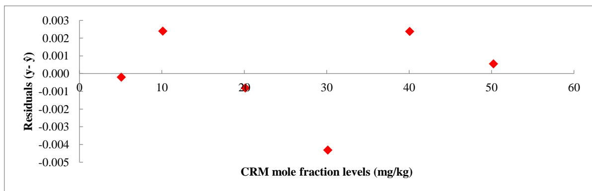
Figure 3. Residuals of the calibration points around an axis 0
