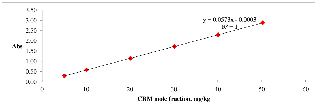
Figure 2. The calibration line of the UV-VIS-NIR spectrophotometer
