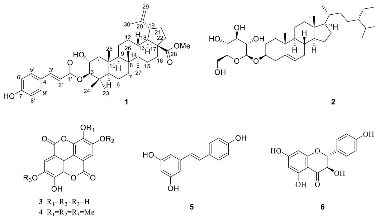
Figure 1. Structures of compounds 1–6 from the roots of A. grossedentata
