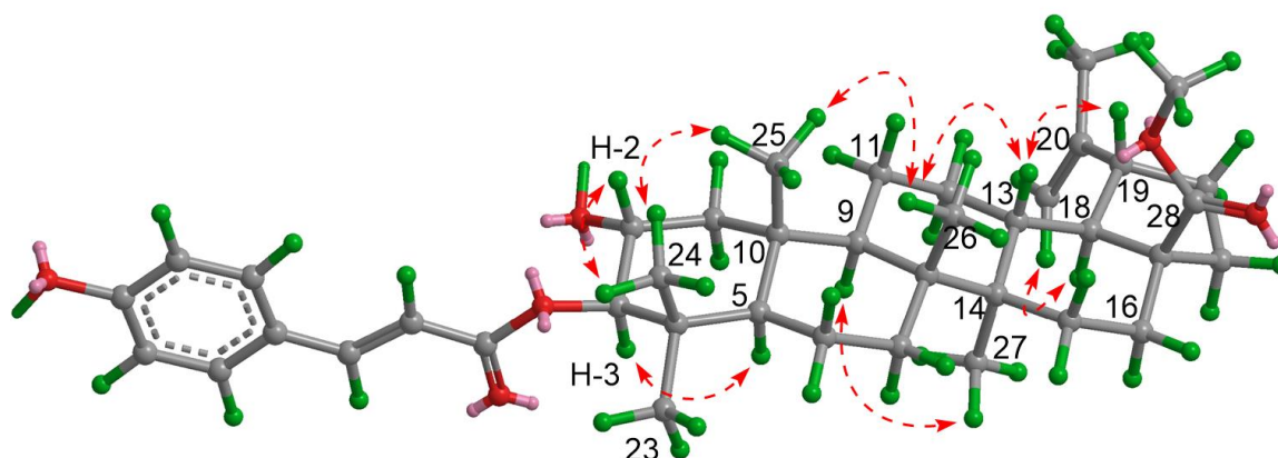
Figure 3. Key NOESY correlations (↔) of 1 .
