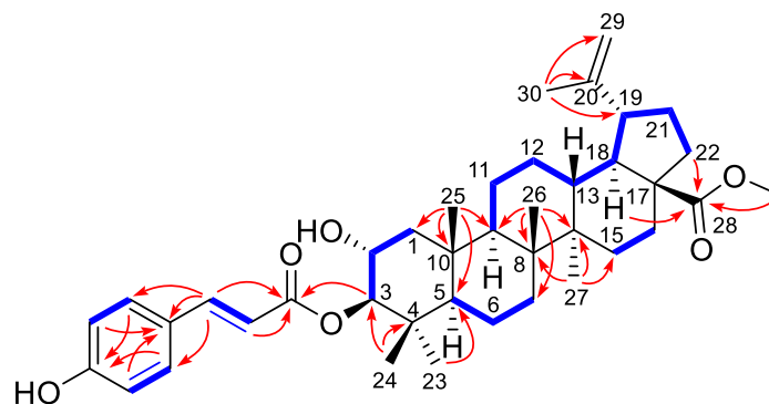
Figure 2. Key COSY (—) and HMBC (→) correlations of 1 .
