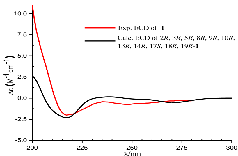
Figure 4. Experimental ECD spectrum of 1 in MeOH and the calculated ECD spectrum of the model molecule 2R , 3R , 5R , 8R , 9R , 10R , 13R , 14R , 17S , 18R , and 19R-1 at the B3LYP/6-31G* in MeOH.
