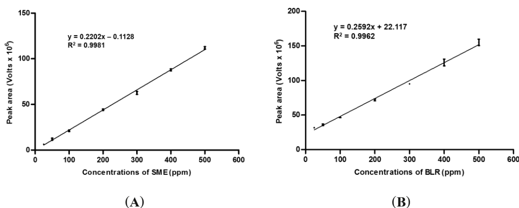
Figure 2. Calibration curve of (A) Shenzhiside methyl ester (SME), (B) Barlerin (BLR)
