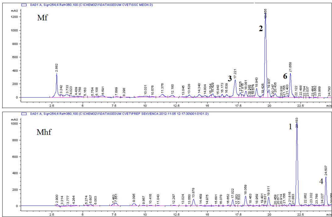
S1: HPLC chromatograms of H. spectabile x telephium flower (Mf) methanol extract and its hydrolysate (Mhf).
