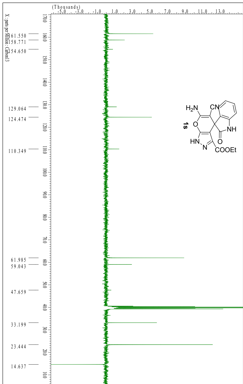
Figure S17. ^{13}\text{C} NMR data of compound 1s
