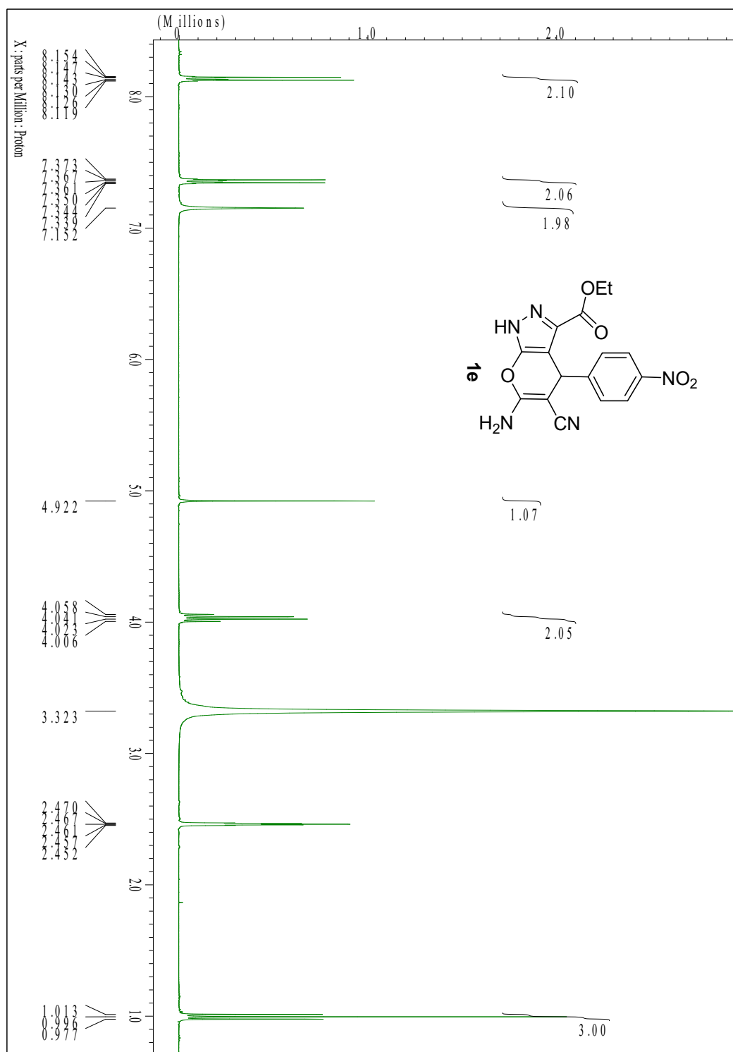
Figure S3. ^1\text{H} NMR data of compound 1e
