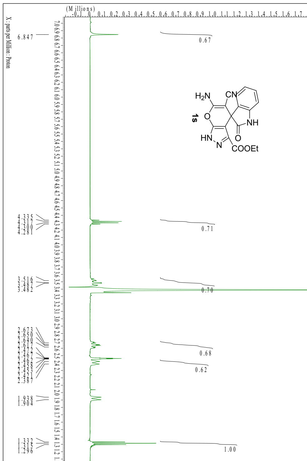
Figure S16. 1 H NMR data of compound 1s
