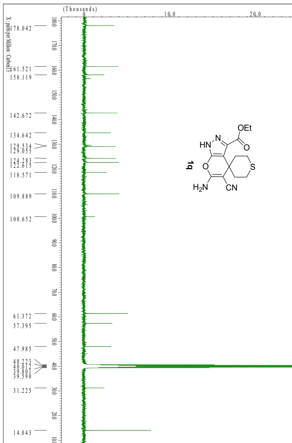
Figure S13. ^{13}\text{C} NMR data of compound 1q
