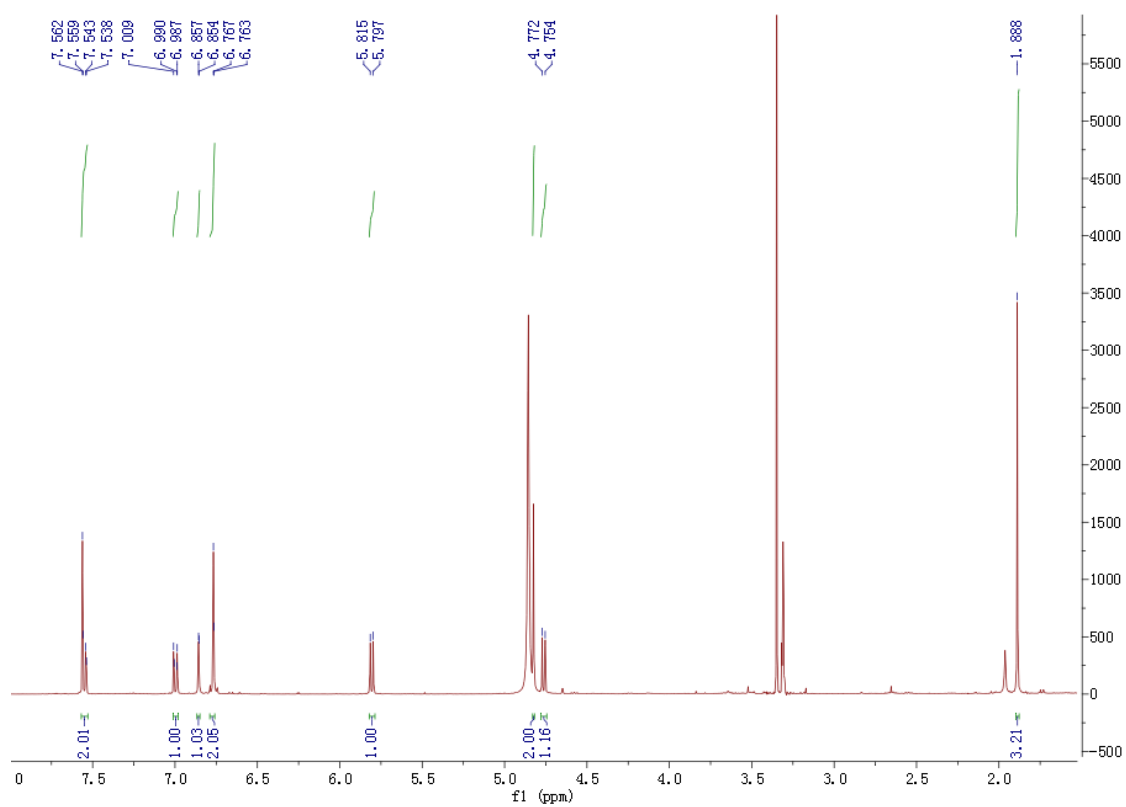
Figure S2: ^1\text{H} -NMR (400 MHz, \text{CD}_3\text{OD} ) Spectrum of 1 (cotidione A)
