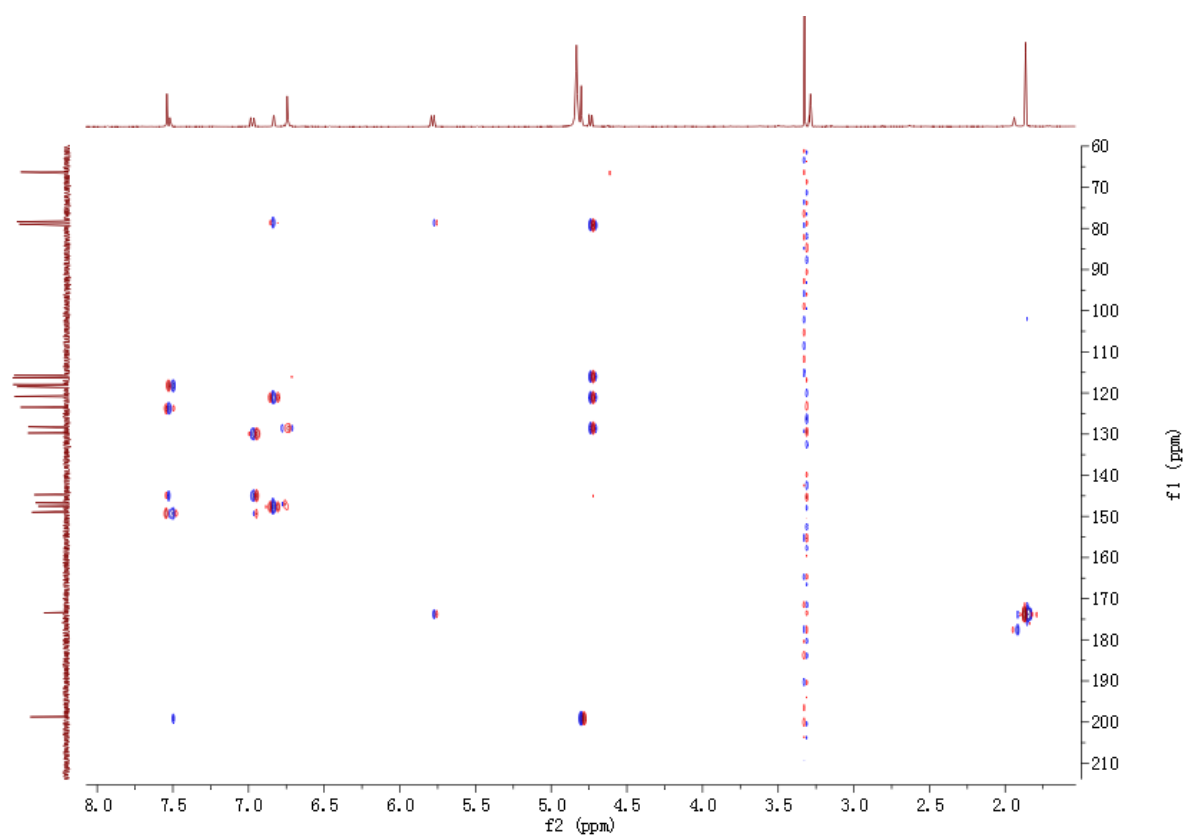
Figure S5: HMBC Spectrum of 1 (cotidione A)
