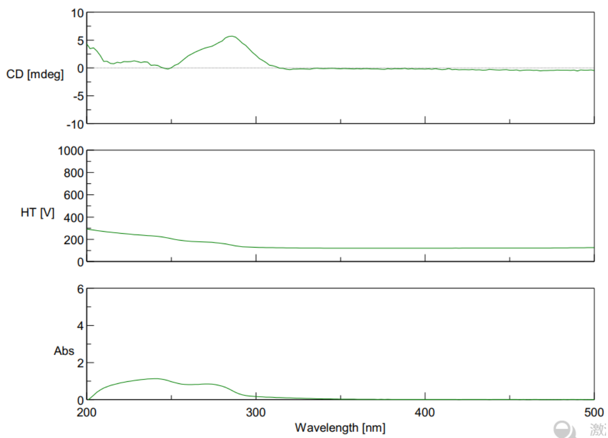
Figure S6: CD Spectrum of 1 (cotidione A)
