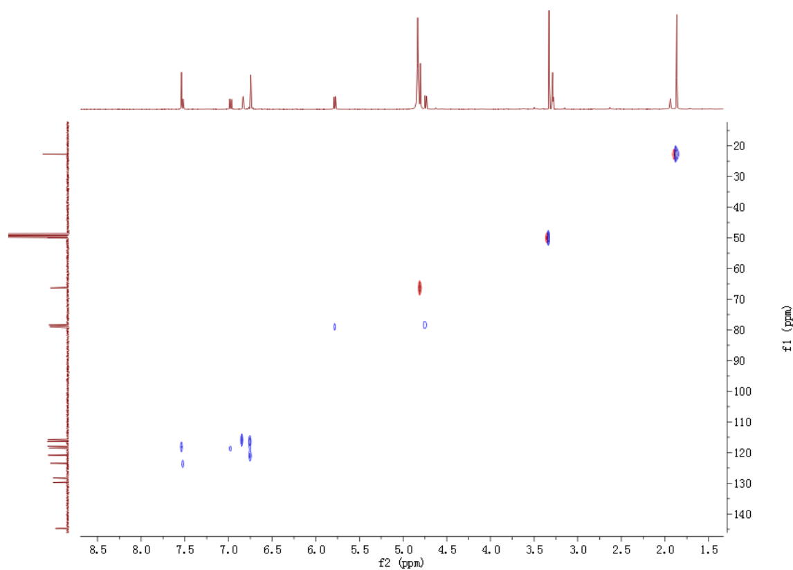
Figure S4: HSQC Spectrum of 1 (cotidione A)
