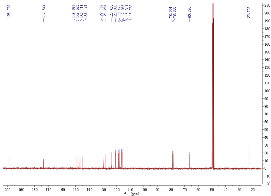
Figure S3: ^{13}\text{C} -NMR (100 MHz, \text{CD}_3\text{OD} ) Spectrum of 1 (cotidione A)
