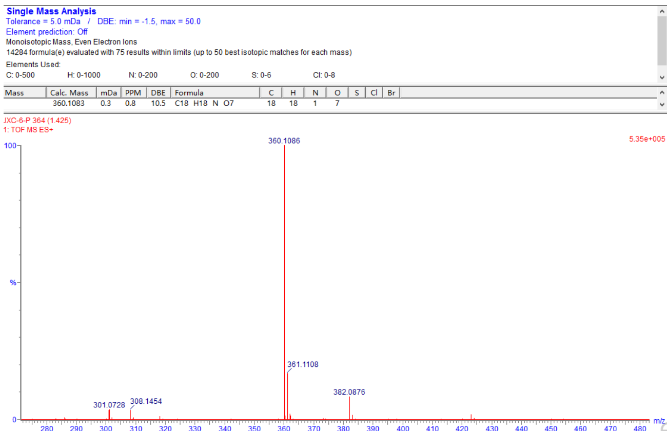
Figure S1: HR-ESI-MS Spectrum of 1 (cotidione A)
