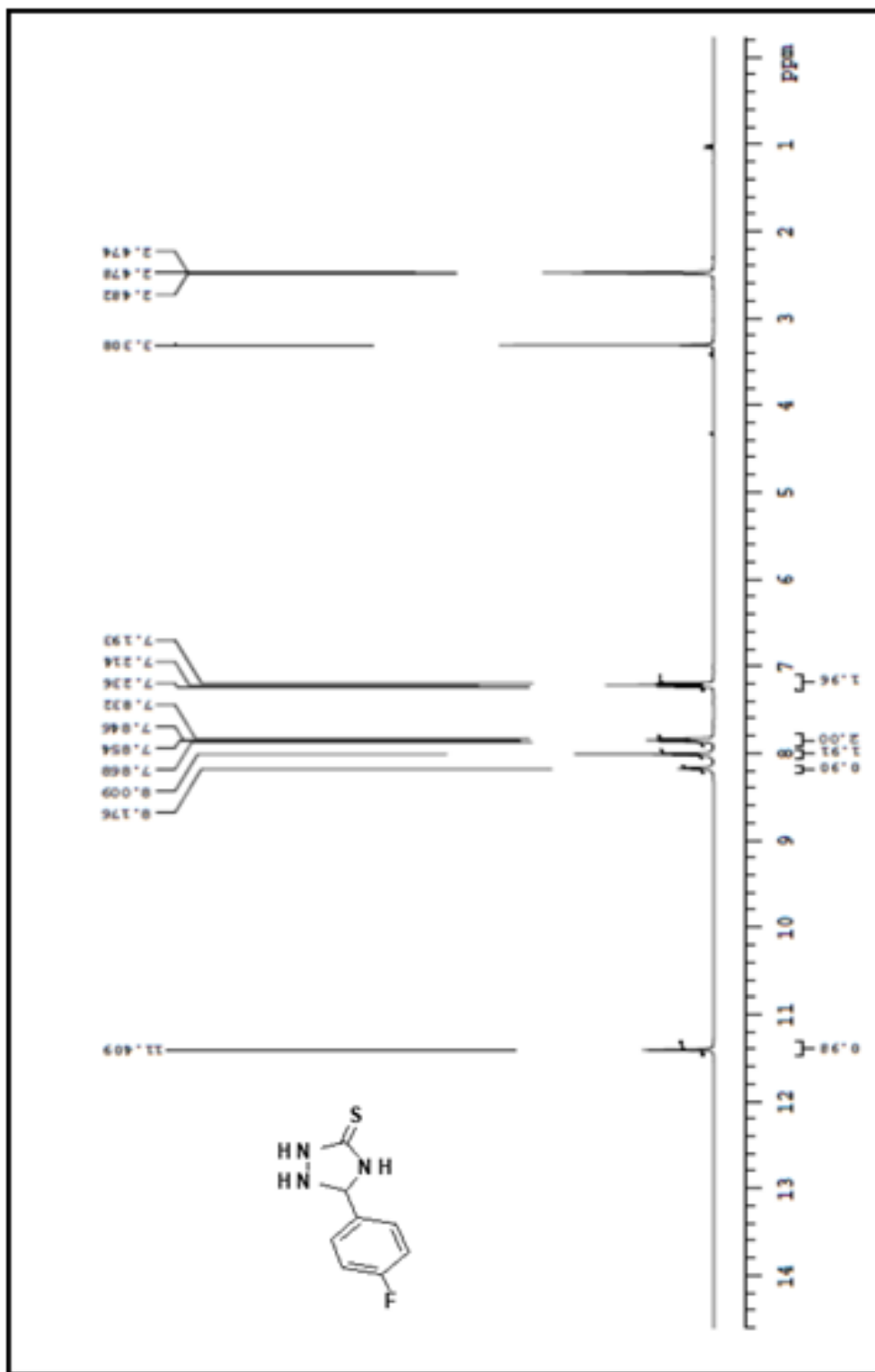
Figure S2: ^1\text{H-NMR} spectrum of 5-aryl-1,2,4-triazolidine-3-thiones (3c)
