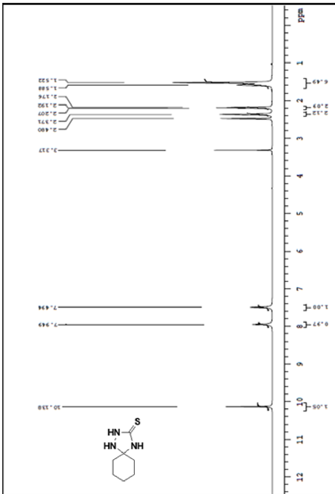
Figure S10: 1 H-NMR Spectrum of 5-aryl-1,2,4-triazolidine-3-thiones (5a)
