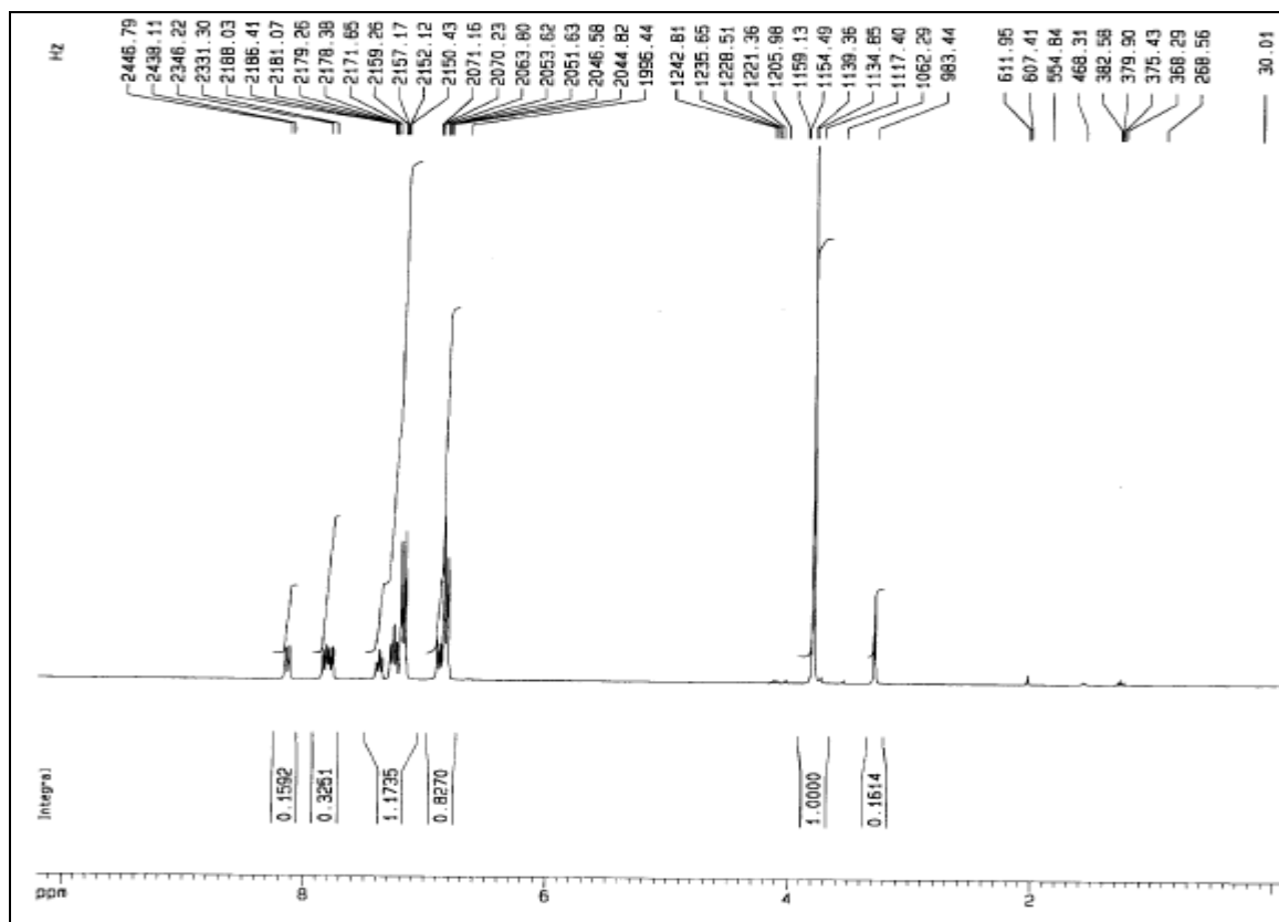
Figure S1: 1 H-NMR spectrum of 2-naphthlene-4,4'-dimethoxy diphenylmethyl alcohol ( 1 )
