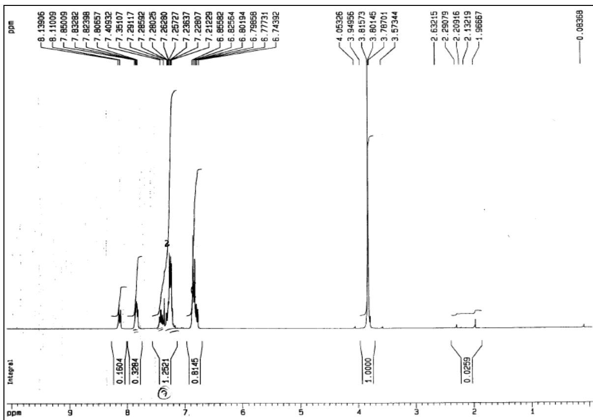
Figure S13: 1 H-NMR spectrum of 1-(chlorobis(4-methoxyphenyl)methyl)naphthalene (9)
