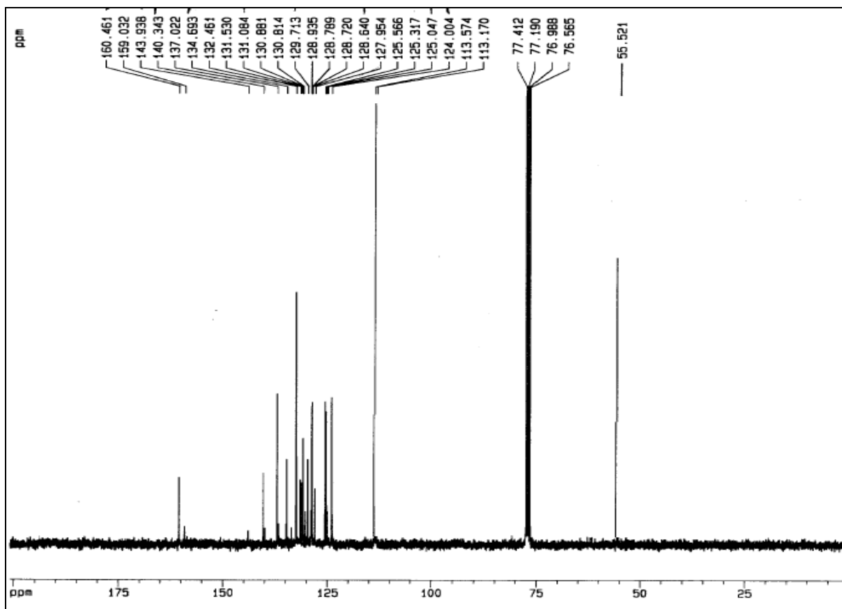
Figure S14: ^{13}\text{C} -NMR spectrum of 1-(chlorobis(4-methoxyphenyl)methyl)naphthalene ( 9 )
