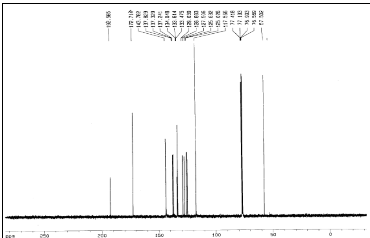
Figure S6: ^{13}\text{C} -NMR spectrum of 1-naphthalene-4,4'-dimethoxydiphenylmethyl tetrafluoroborate ( 4 )
