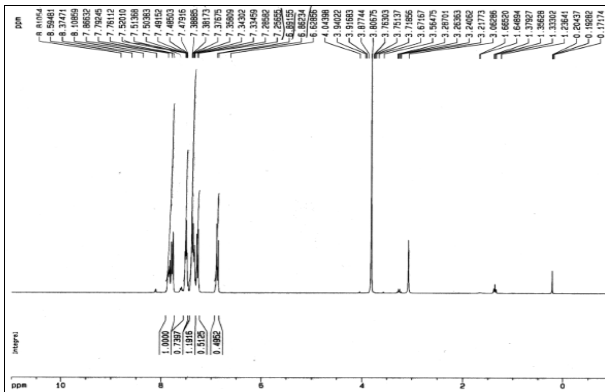
Figure S7: 1 H-NMR spectrum of 2-naphthyl-4-monomethoxy diphenylmethyl alcohol (5)
