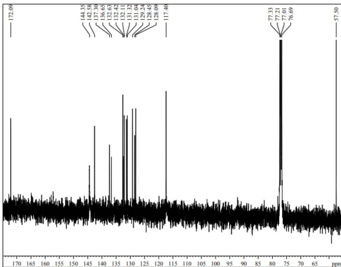
Figure S4: ^{13}\text{C} -NMR spectrum of 2-naphthalene-4,4'-dimethoxydiphenylmethyl tetrafluoroborate (2)
