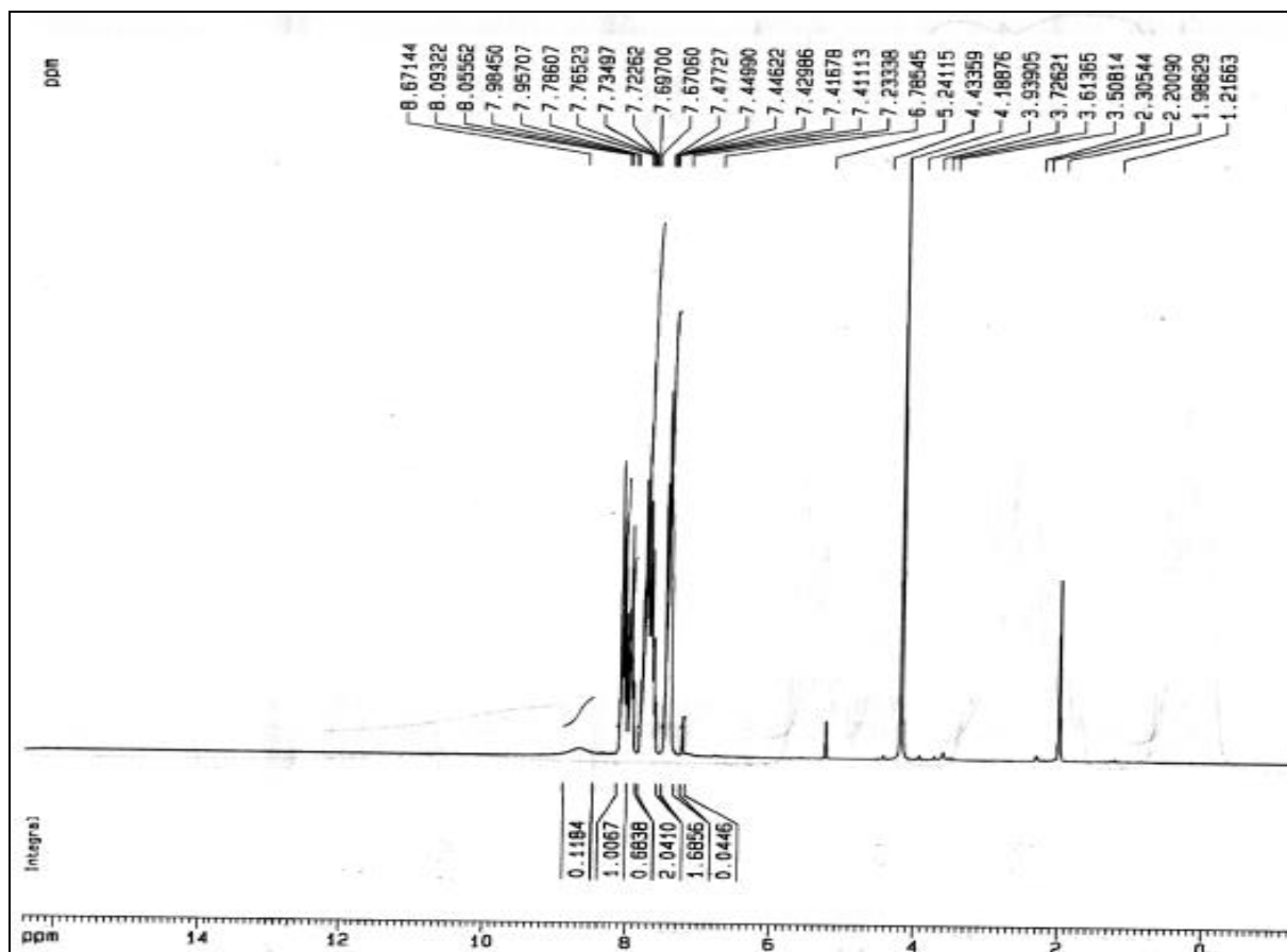
Figure S9: 1 H-NMR spectrum of 2-naphthalene-4-monomethoxydiphenylmethyl tetrafluoroborate ( 6 )
