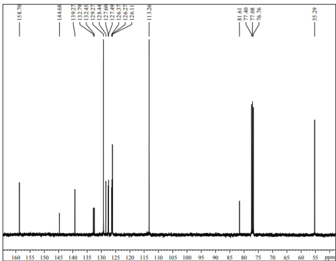
Figure S2: ^{13}\text{C} -NMR spectrum of 2-naphthyl-4,4'-dimethoxydiphenylmethyl alcohol ( 1 )
