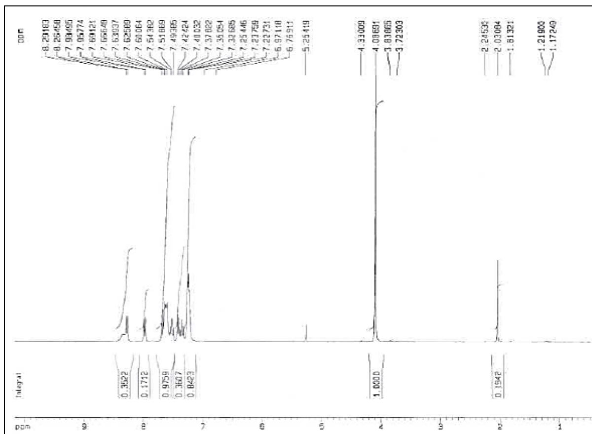
Figure S5: 1 H-NMR spectrum of 1-naphthalene-4,4'-dimethoxydiphenylmethyl tetrafluoroborate ( 4 )
