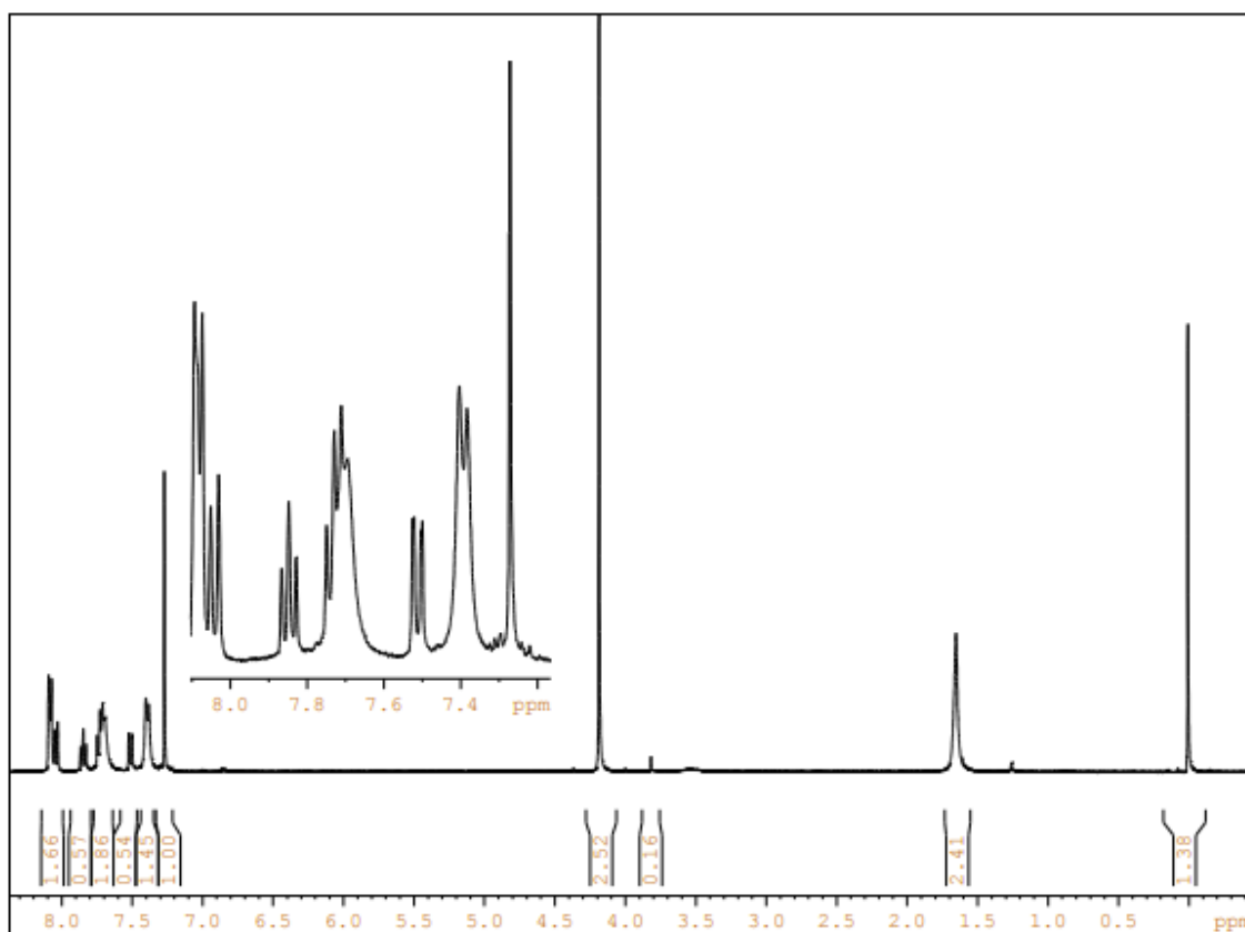
Figure S3: ^1\text{H-NMR} spectrum of 2-naphthalene-4,4'-dimethoxydiphenylmethyl tetrafluoroborate (2)
