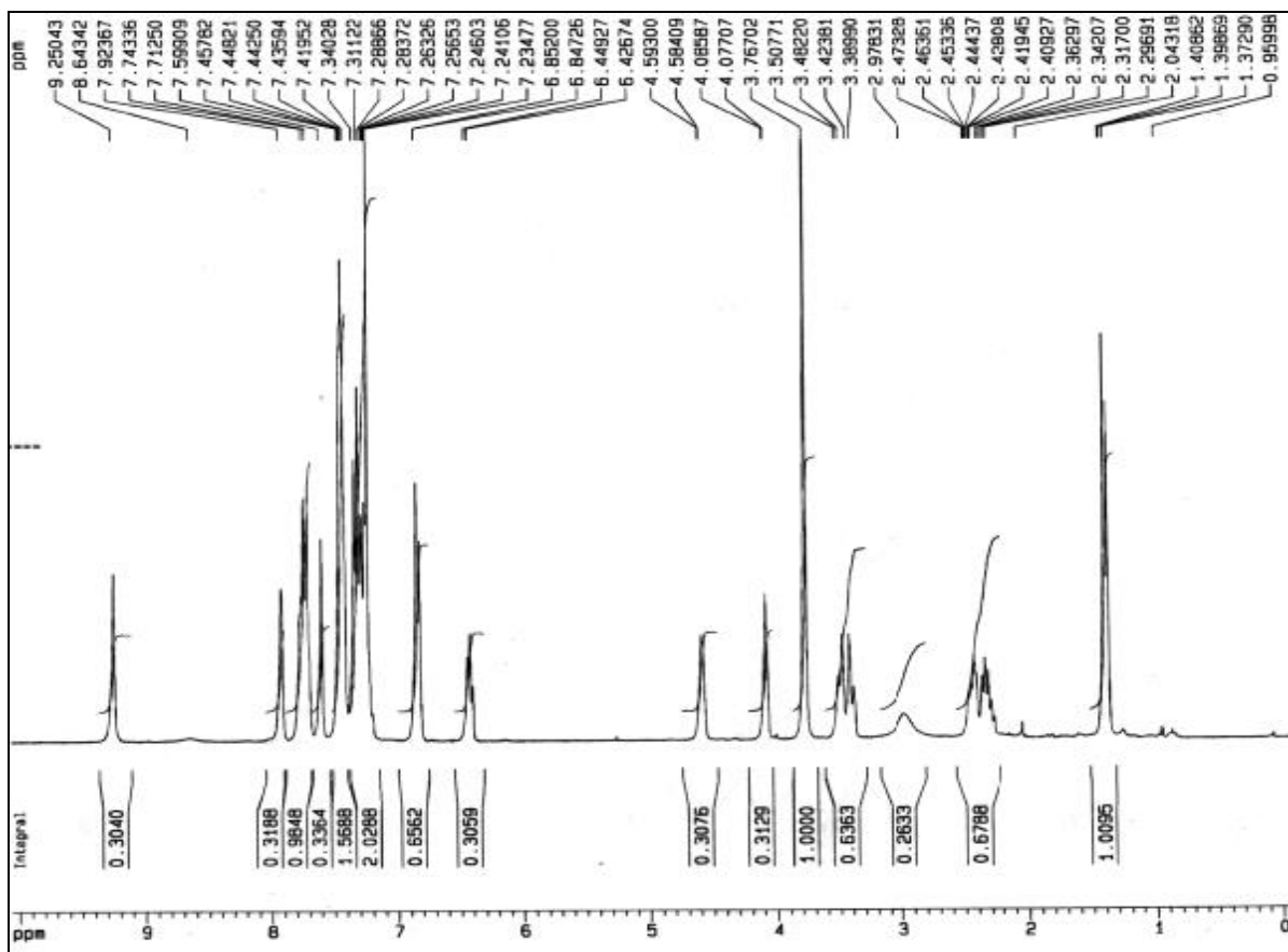
Figure S15: 1 H-NMR spectrum of O-5'-(2-naphthalene-4-monomethoxydiphenylmethyl)thymidine (11)
