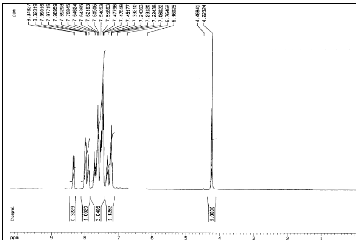
Figure S11: ^1\text{H-NMR} spectrum of 1-naphthalene-4-monomethoxydiphenylmethyl tetrafluoroborate ( 8 )
