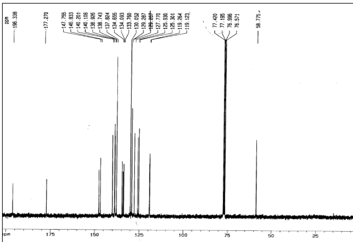
Figure S12: ^{13}\text{C} -NMR spectrum of 1-naphthalene-4-monomethoxydiphenylmethyl tetrafluoroborate ( 8 )
