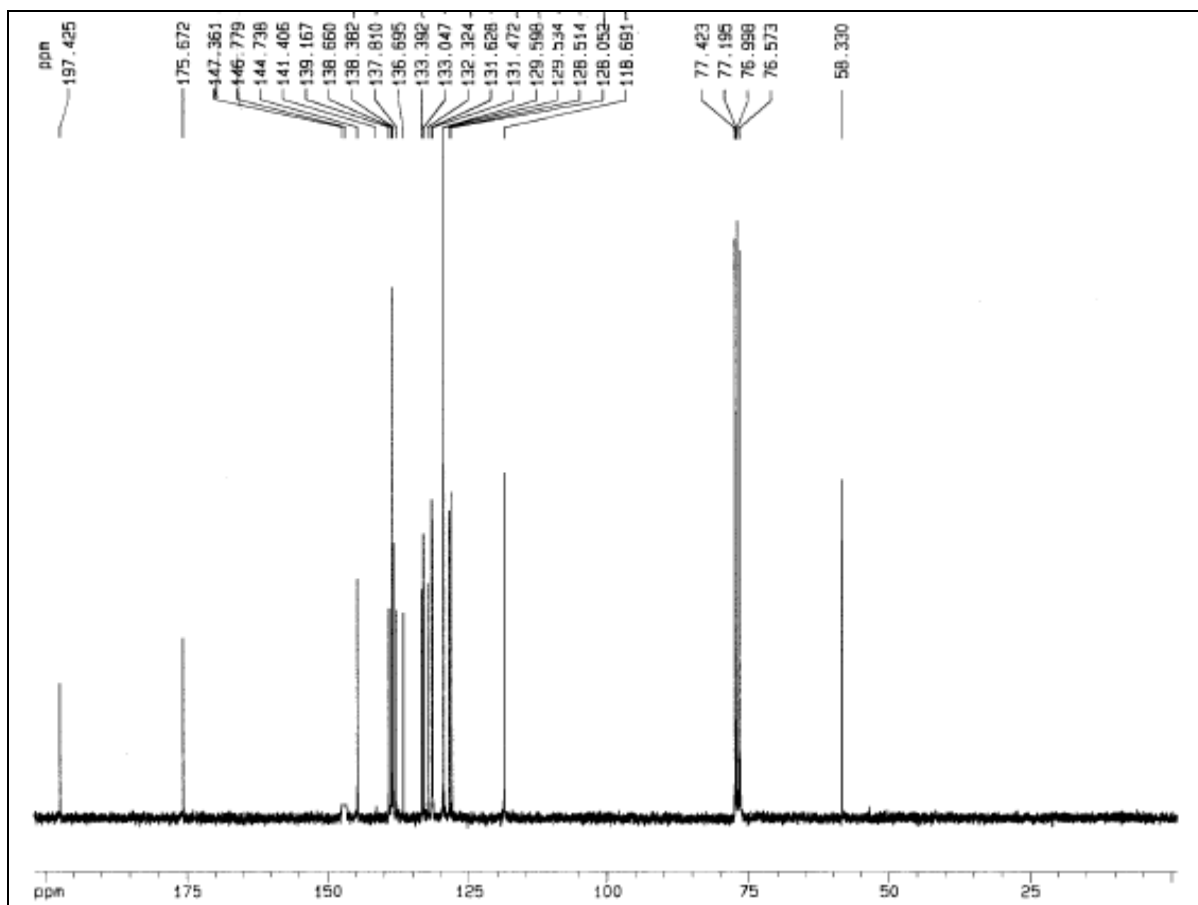
Figure S10: ^{13}\text{C} -NMR spectrum of 2-naphthalene-4-monomethoxydiphenylmethyl tetrafluoroborate ( 6 )
