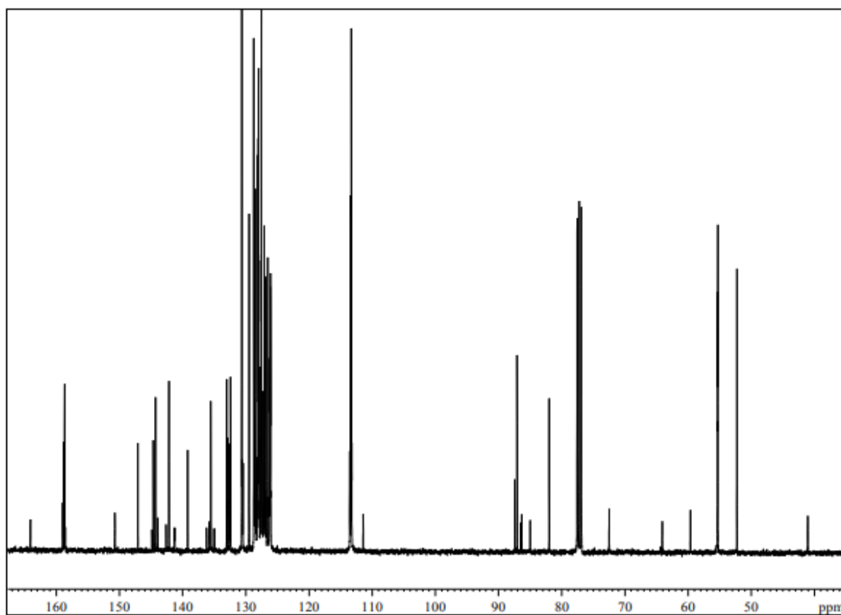
Figure S16: ^{13}\text{C} -NMR spectrum of O-5'-(2-naphthalene-4-monomethoxydiphenylmethyl)thymidine ( 11 )
