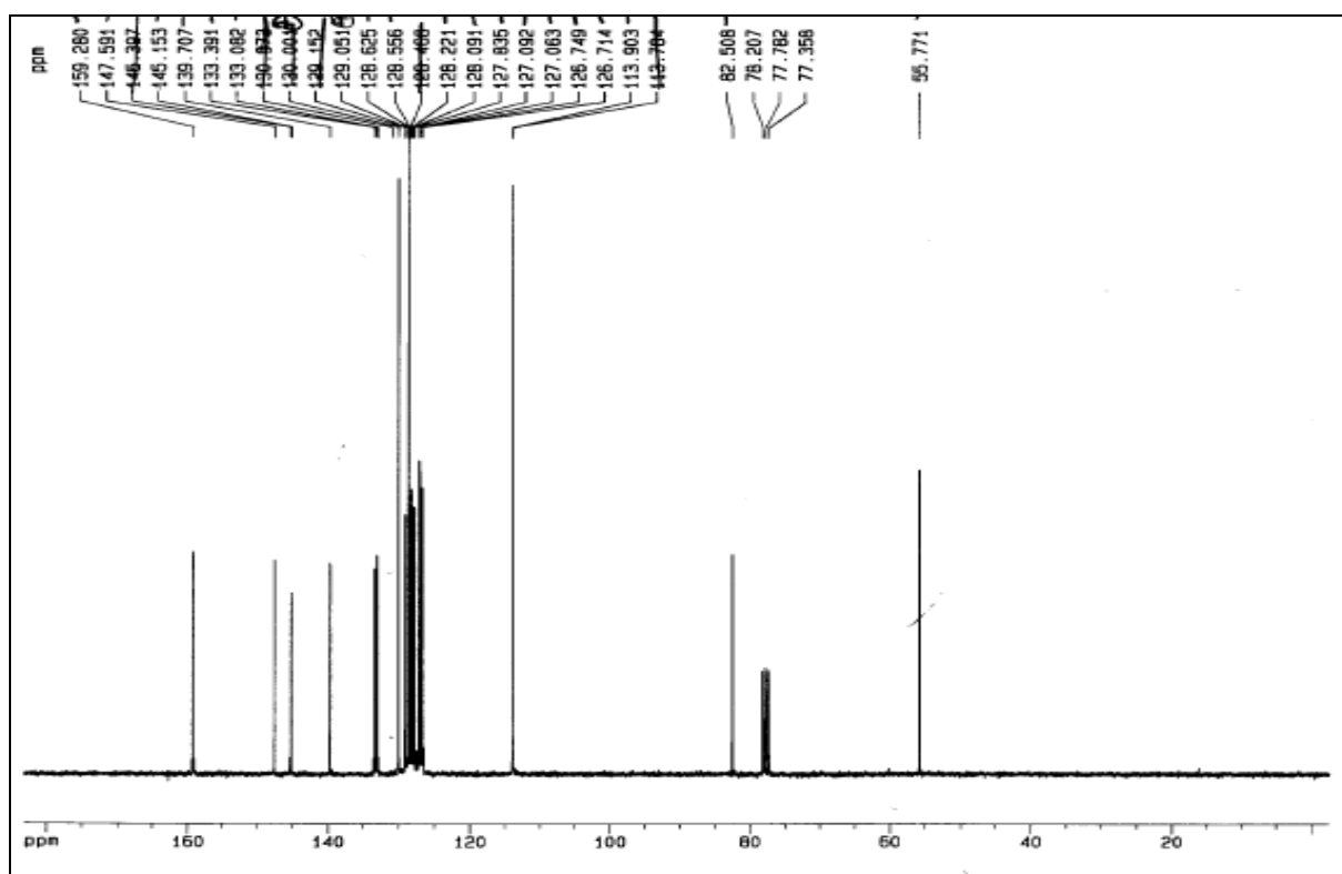
Figure S8: ^{13}\text{C} -NMR spectrum of 2-naphthyl-4-monomethoxy diphenylmethyl alcohol ( 5 )
