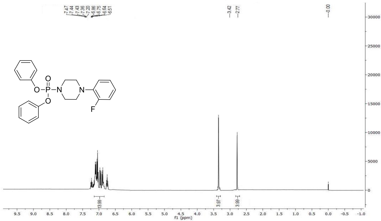
Figure S3: 1 H NMR Spectrum of compound 3f
