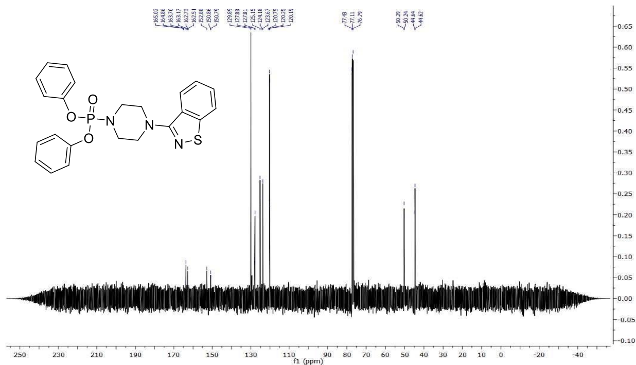
Figure S2: ^{13}\text{C} NMR Spectrum of compound 3a
