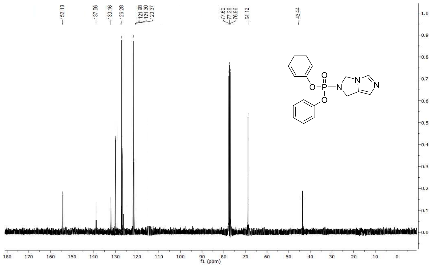
Figure S8: 13 C NMR Spectrum of compound 3j
