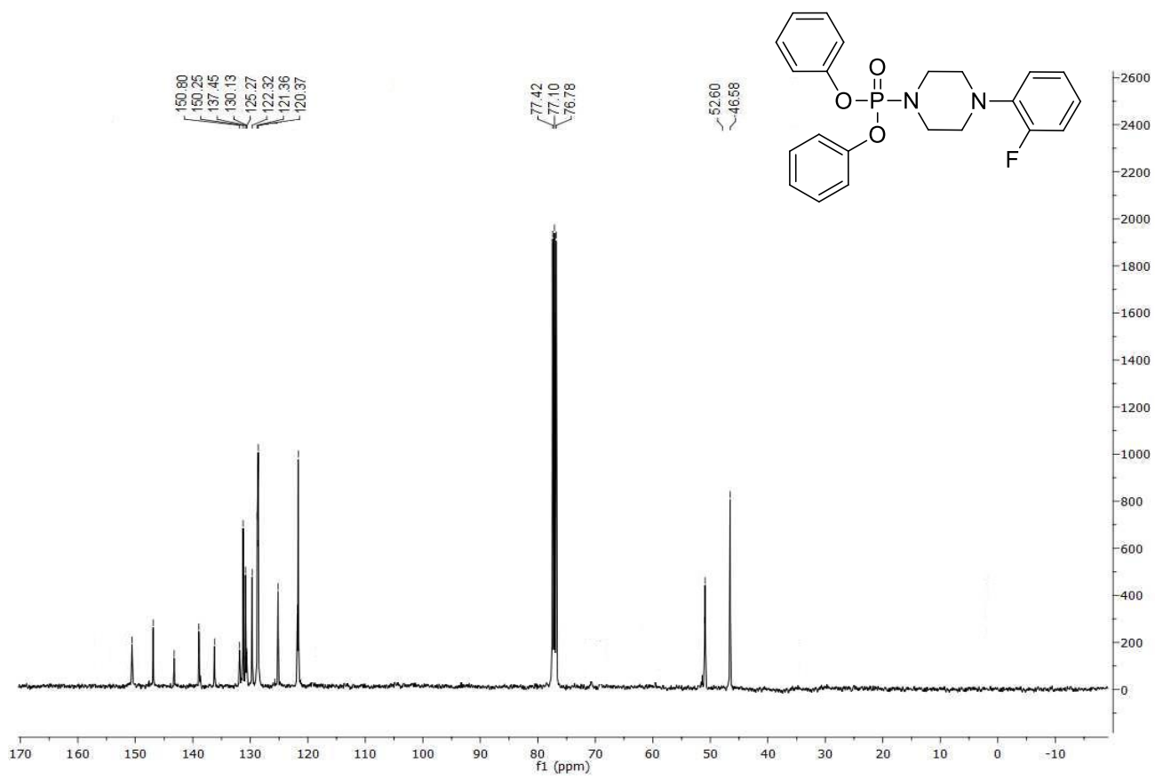
Figure S4: 1 H NMR Spectrum of compound 3f
