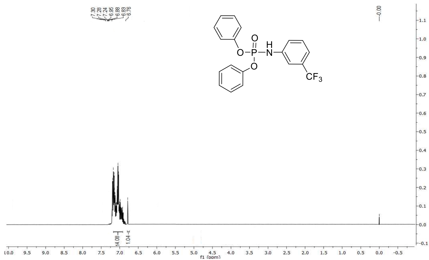
Figure S5: 1 H NMR Spectrum of compound 3i
