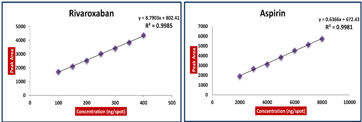
Figure S1: Calibration curve (a) Rivaroxaban (100-400 ng/band) and (b) Aspirin (2000-8000 ng/band)
