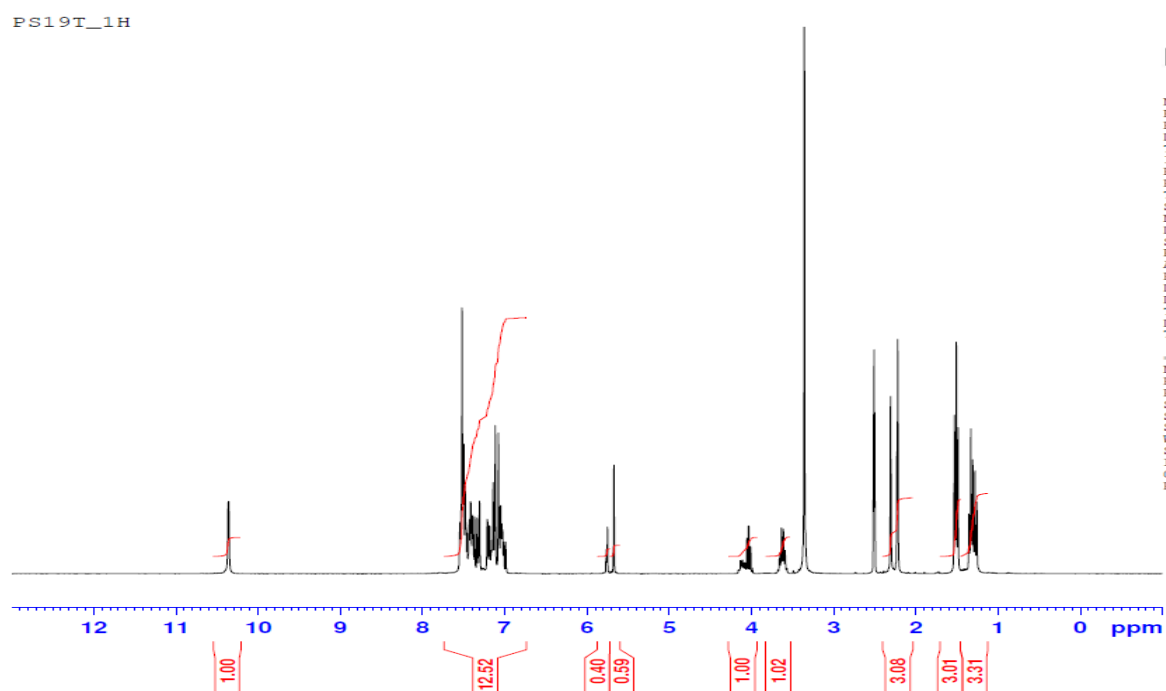
Figure S91: ^1\text{H} -NMR spectrum of the compound 4r
