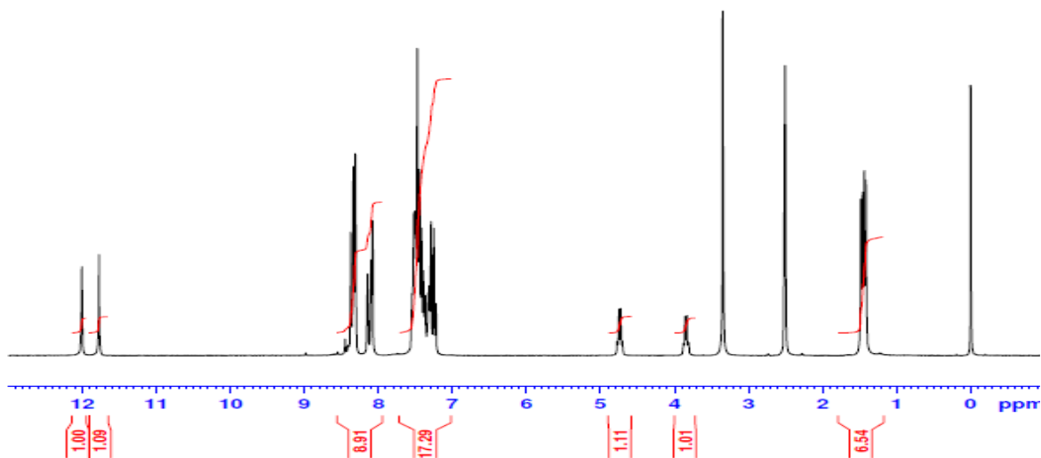
Figure S20: ^1\text{H} -NMR spectrum of the compound 3h
