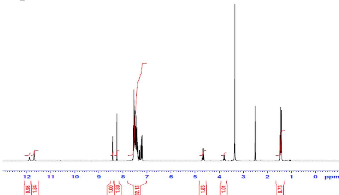
Figure S18: 1 H-NMR spectrum of the compound 3g
