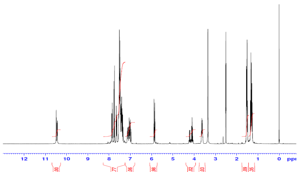
Figure S45: 1 H-NMR spectrum of the compound 4a
