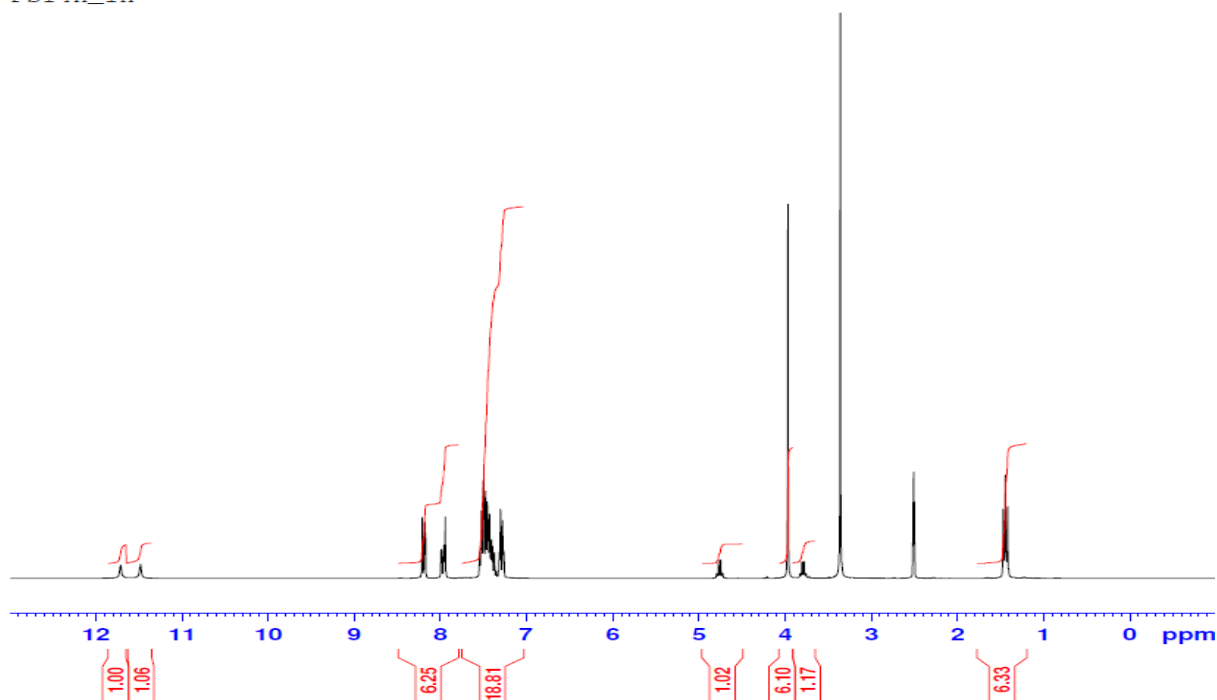
Figure S32: 1 H-NMR spectrum of the compound 31
