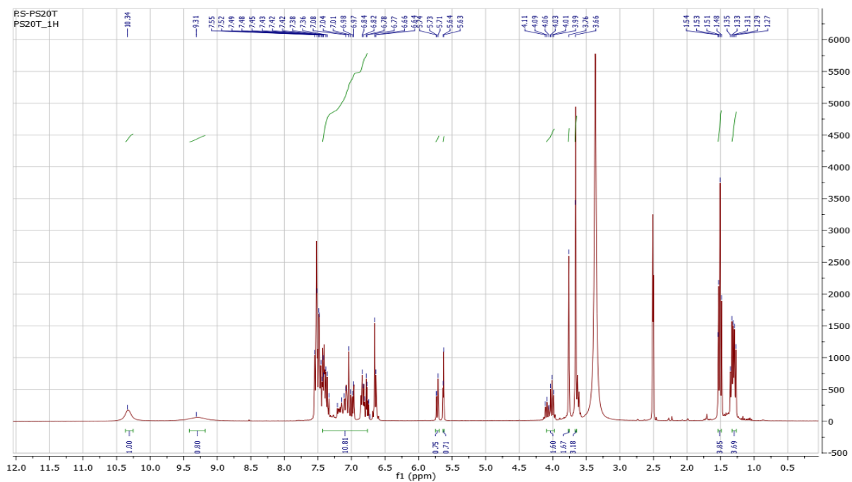
Figure S94: ^1\text{H} -NMR spectrum of the compound 4s
