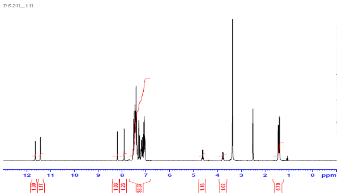
Figure S5: 1 H-NMR spectrum of the compound 3b
