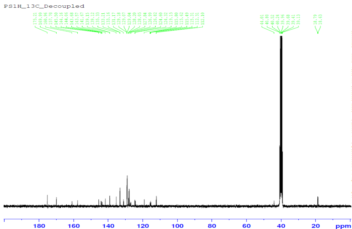
Figure S3: 13 C-NMR spectrum of the compound 3a
