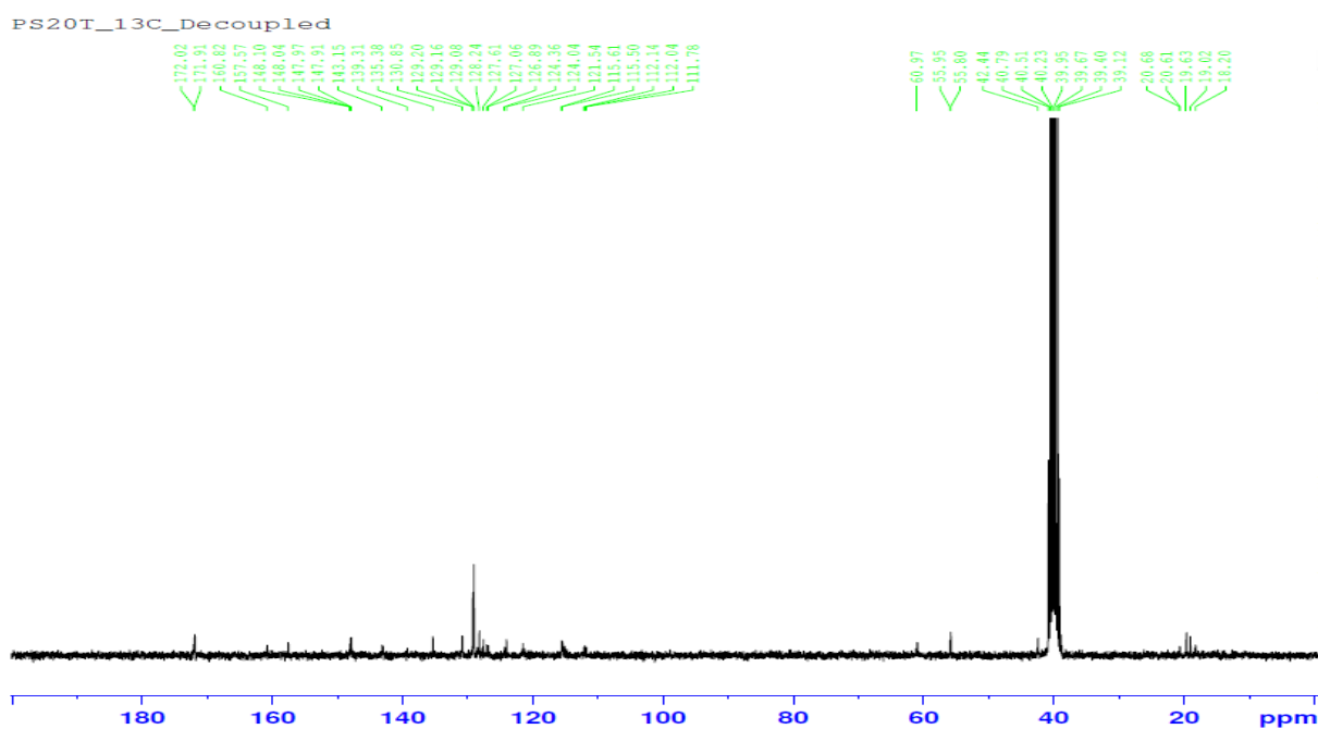
Figure S95: ^{13}\text{C} -NMR spectrum of the compound 4s
